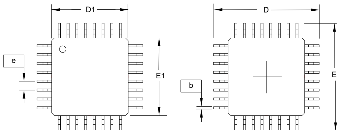
BOTTOM VIEW
