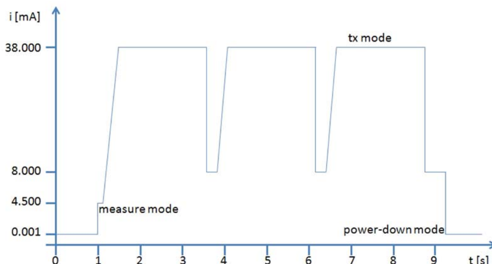
Figure 5-2. Standalone Mode Current Consumption at 24°C
