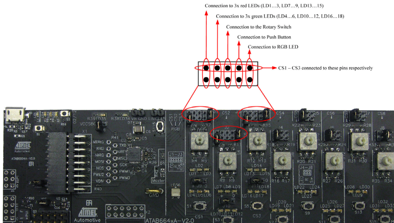
Figure 3-9. Jumpers JP1...3
