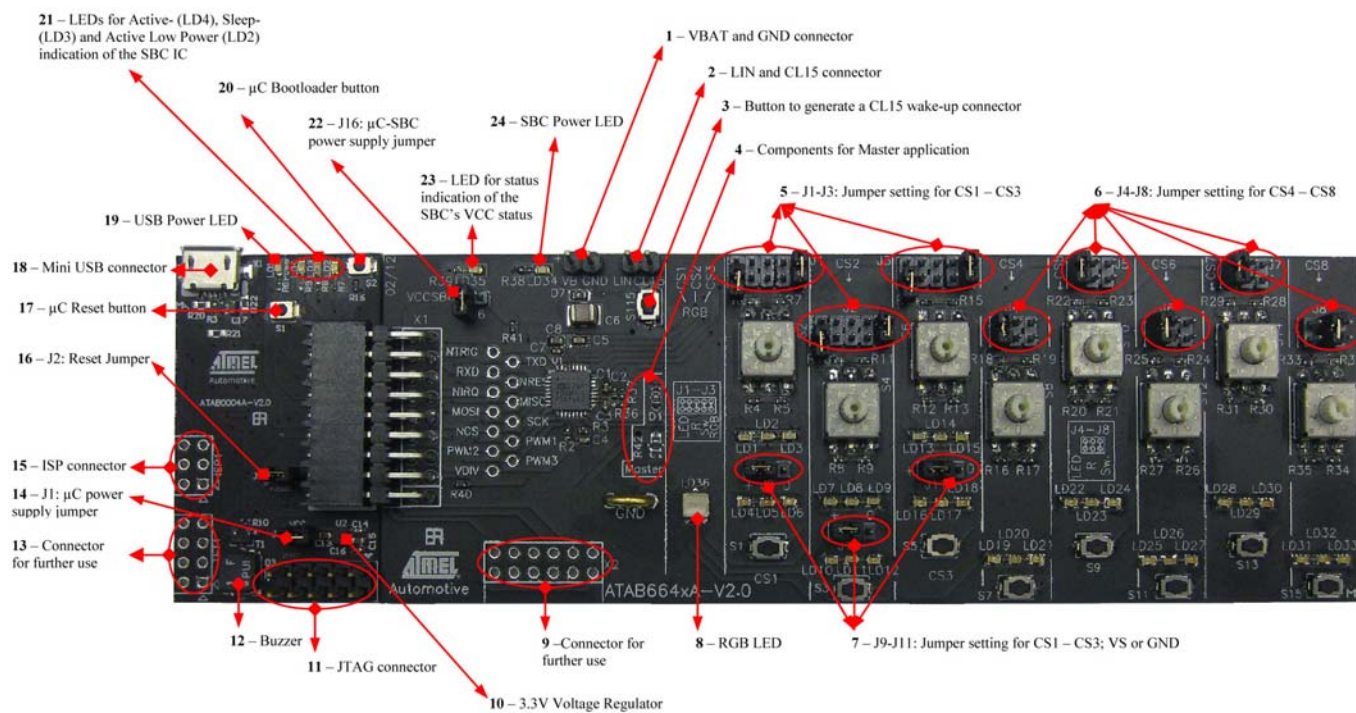
Figure 2-1. Atmel ATA42001-V1 Development Kit with Reference Points
