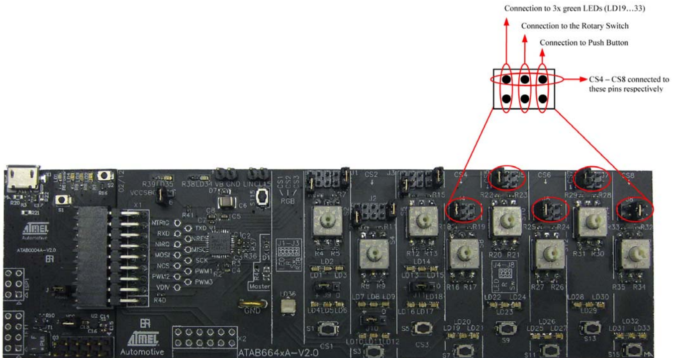
Figure 3-10. Jumpers JP4...8
