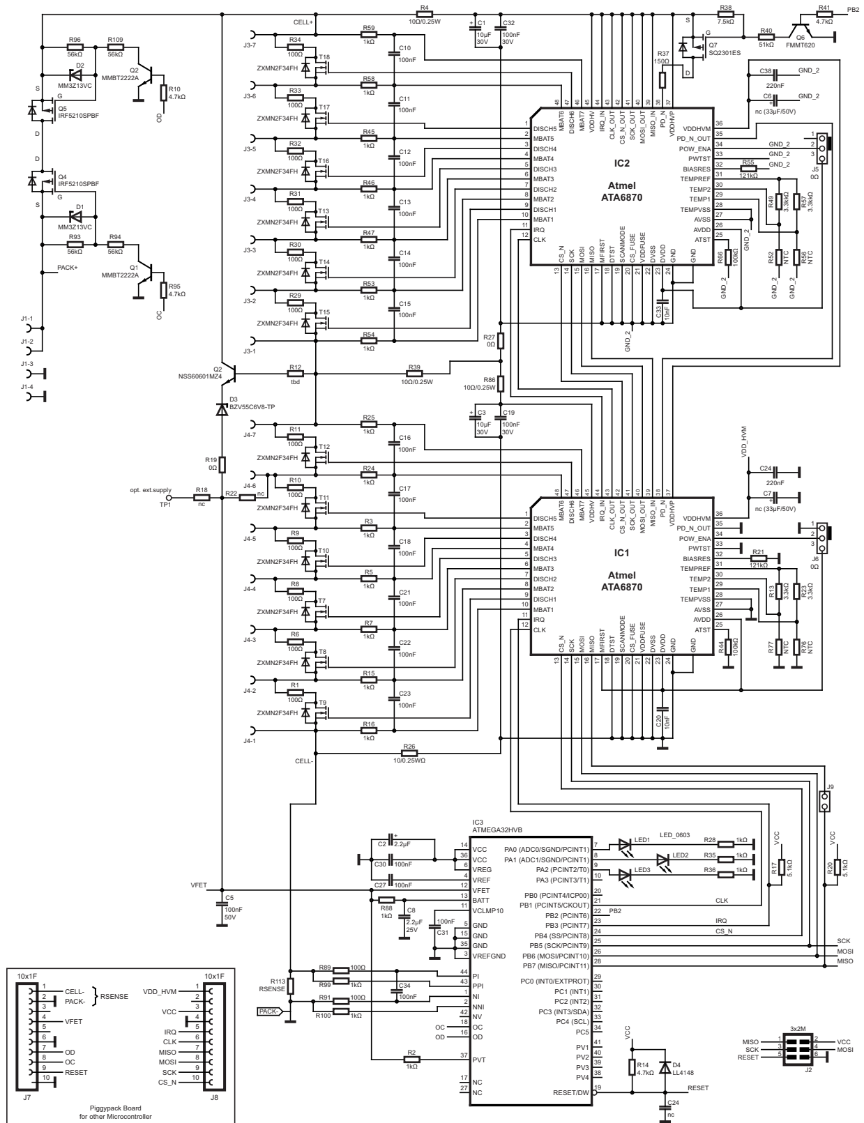
Figure 7-1. Schematic
