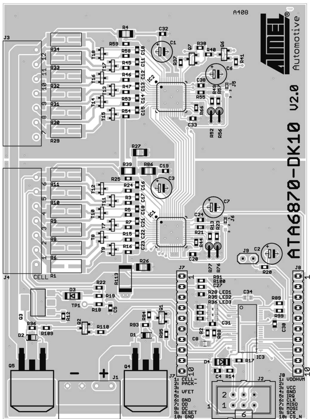
Figure 7-2. PCB Top
