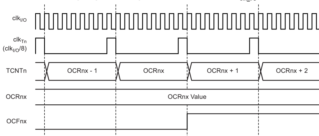
Figure 4-39. Timer/Counter Timing Diagram, Setting of \text{OCF0A} , with Prescaler ( f_{\text{clk}_{I/O}/8} )
