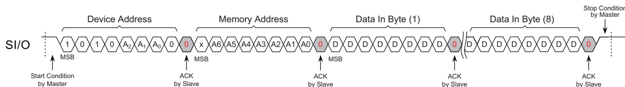
Figure 6-2. Page Write
