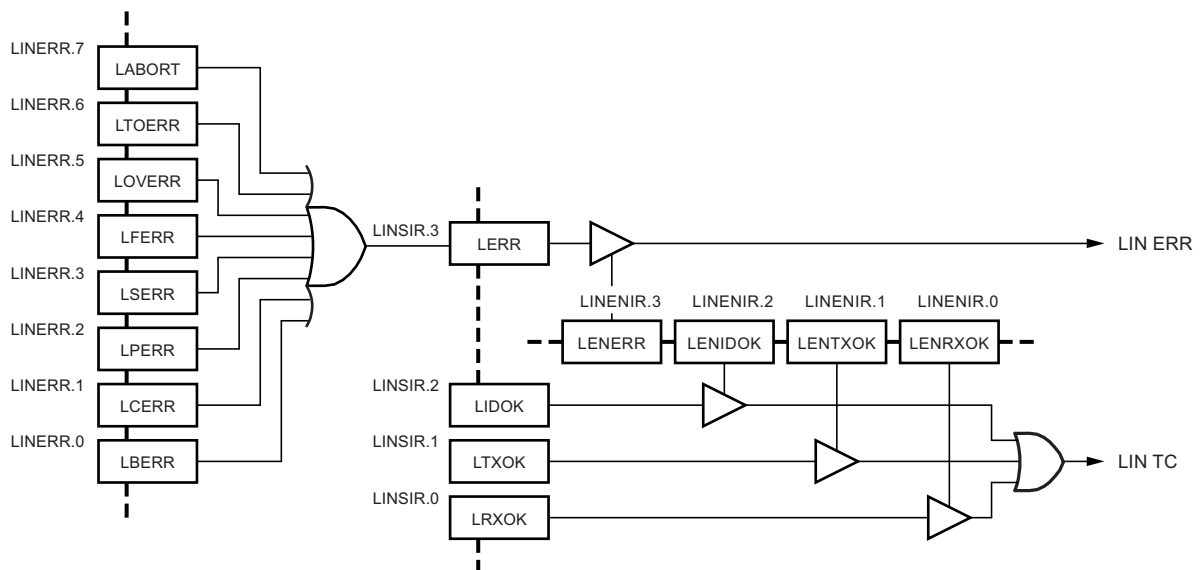
Figure 15-13.LIN Interrupt Mapping
