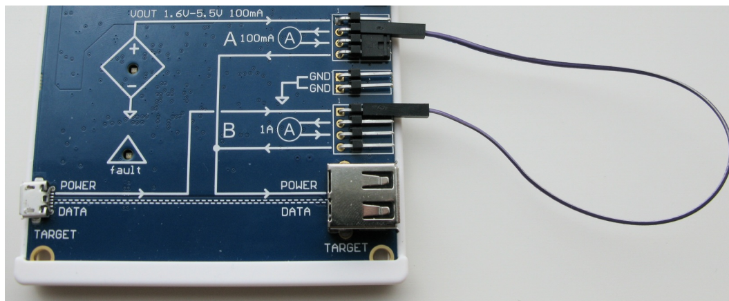
Figure 6-6. Jumper Configuration
