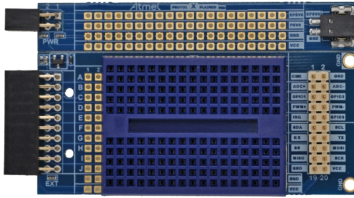
Figure 4-8. Solderless Breadboard Mounted on PROTO1 Xplained Pro
