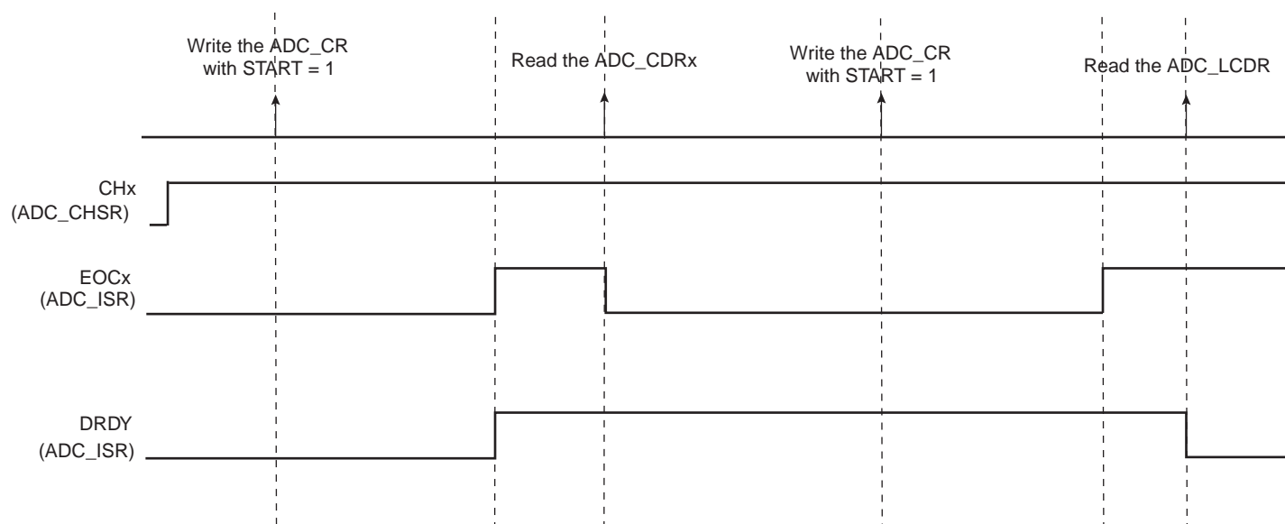
Figure 33-3. EOCx and DRDY Flag Behavior
