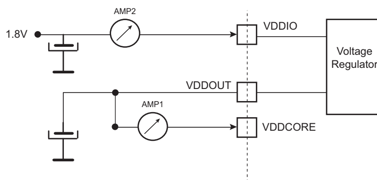
Figure 34-7. Active Mode Measurement Setup
