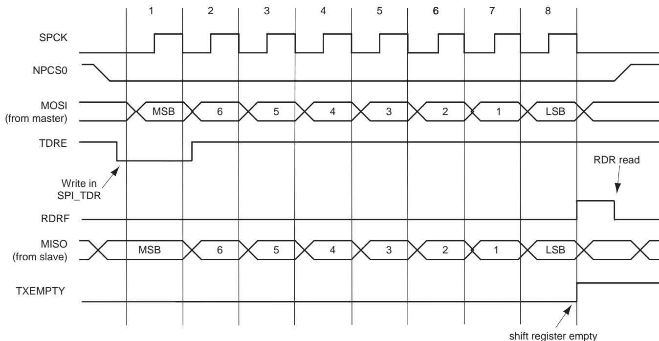
Figure 27-8. Status Register Flags Behavior
