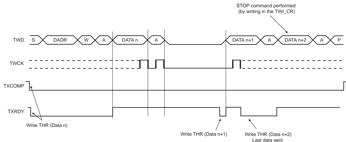
Figure 29-6. Master Write with Multiple Data Bytes
