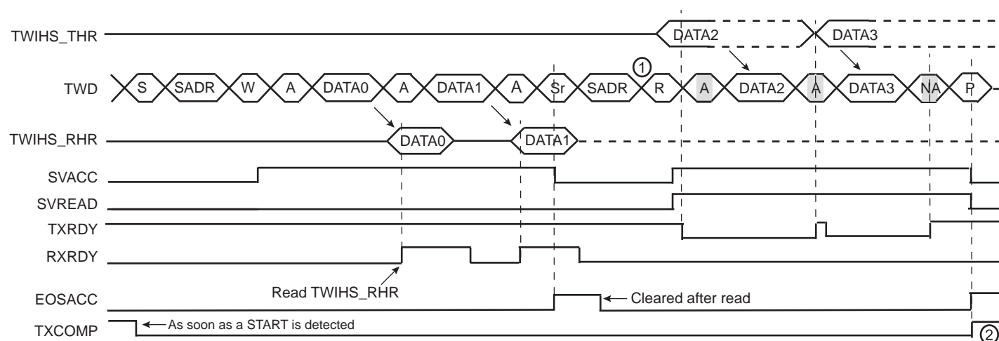
Figure 28-42. Repeated Start and Reversal from Write Mode to Read Mode
