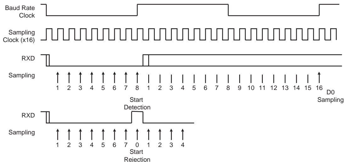
Figure 31-6. Asynchronous Start Detection
