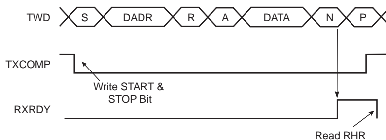
Figure 28-10. Master Read with One Data Byte
