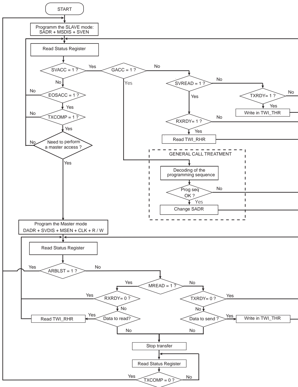
Figure 29-23. Multi-master Flowchart
