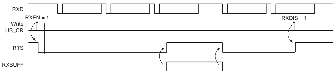
Figure 31-16. Receiver Behavior when Operating with Hardware Handshaking
