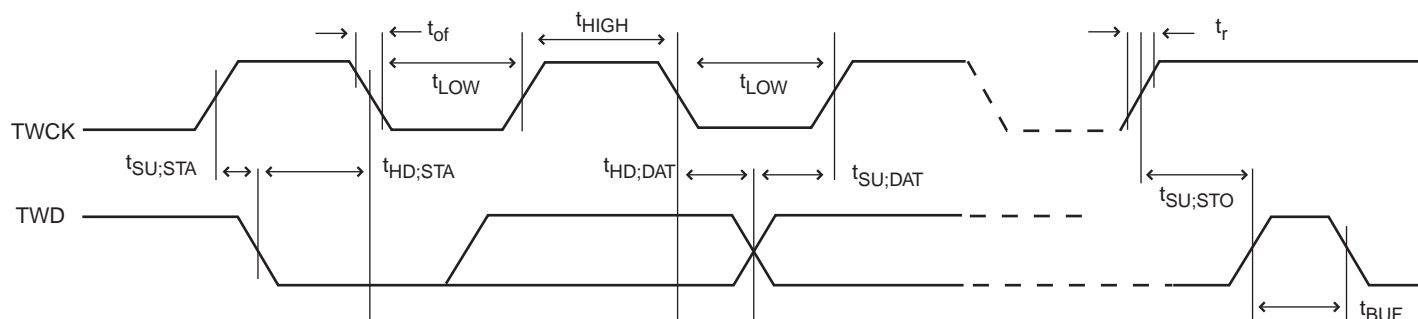
Figure 34-19. Two-wire Serial Bus Timing
