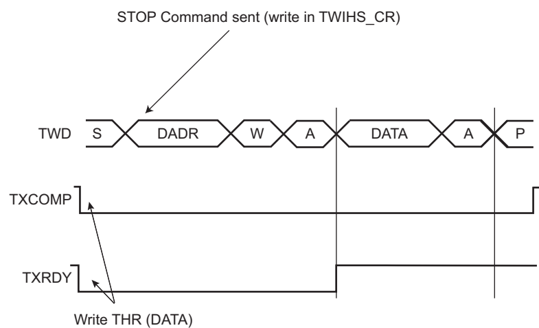
Figure 28-7. Master Write with One Data Byte
