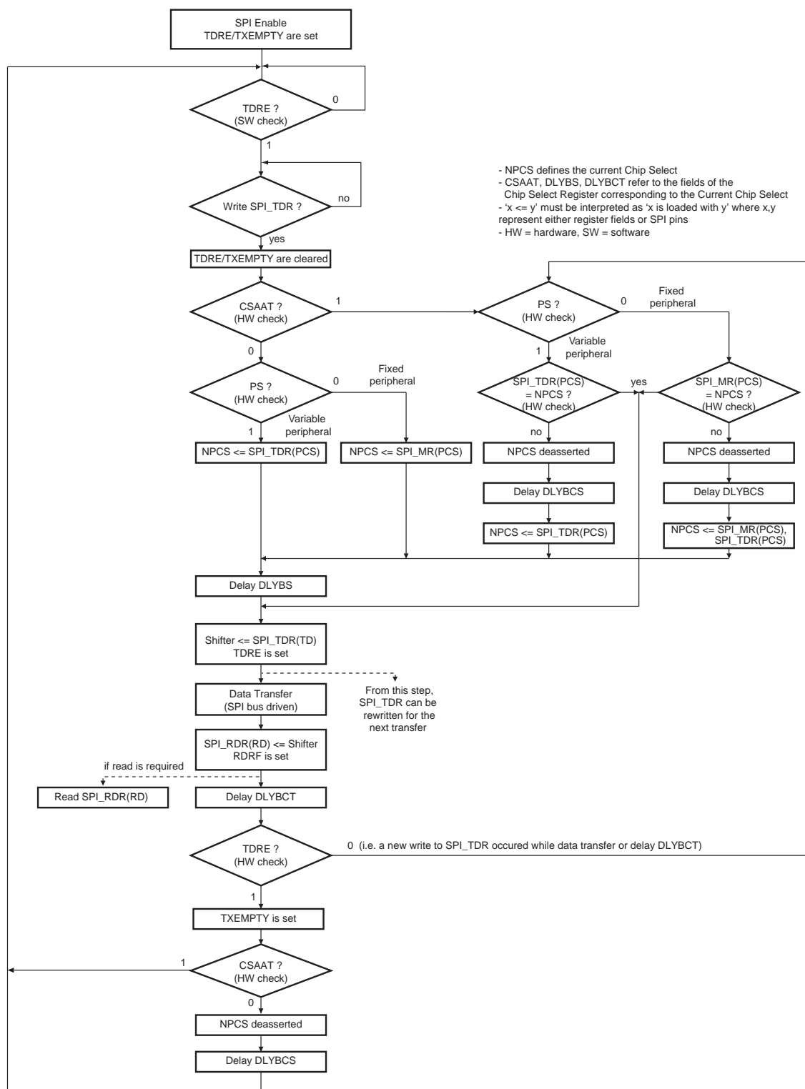
Figure 27-7. Master Mode Flow Diagram
