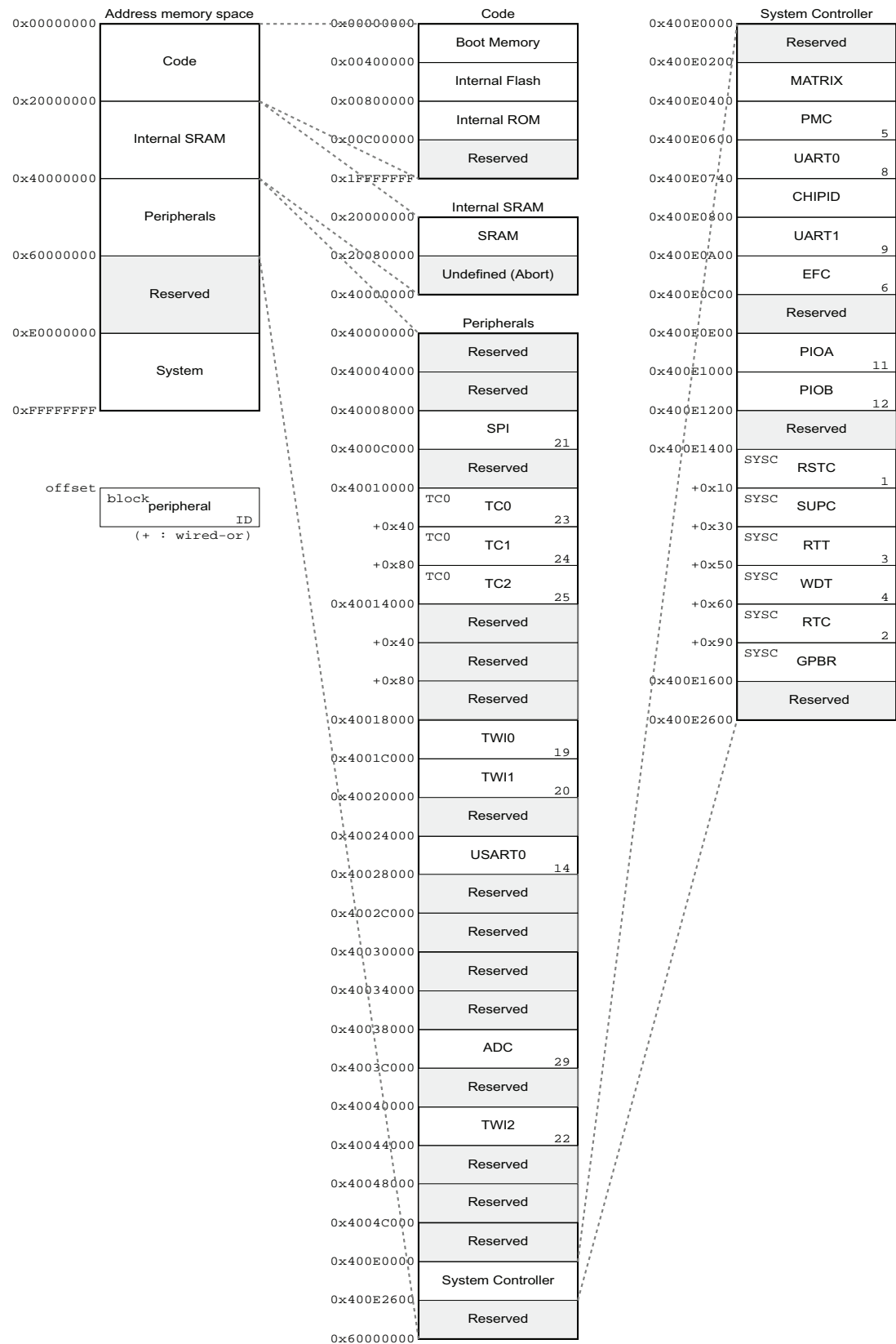
Figure 6-1. SAM G51 Series Product Mapping
