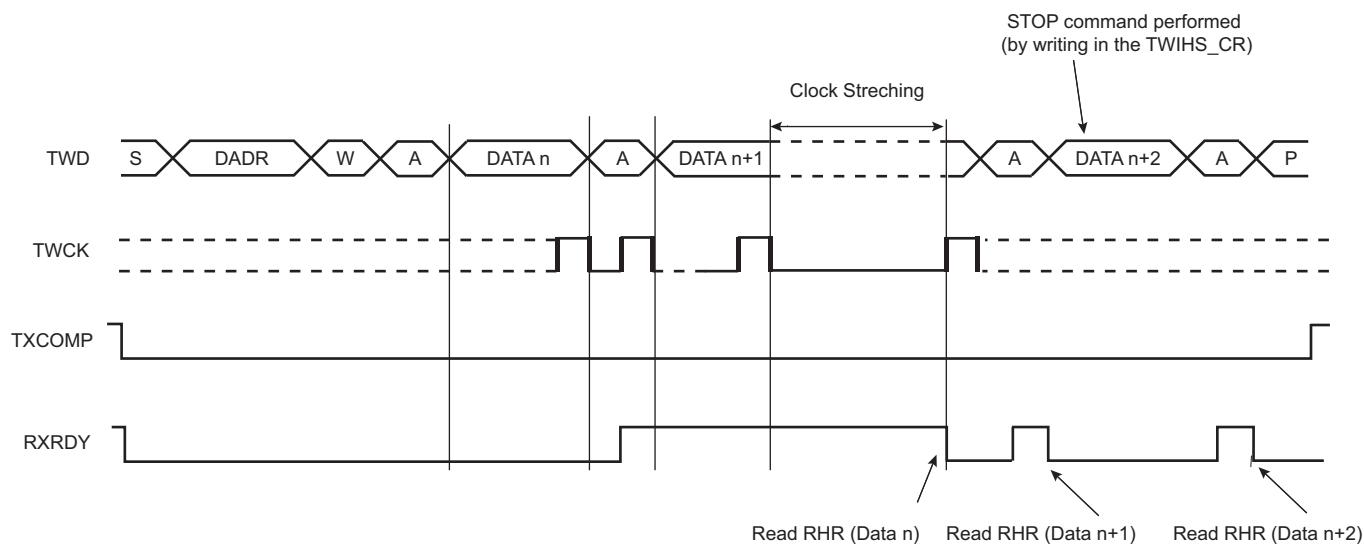
Figure 28-12. Master Read Clock Stretching with Multiple Data Bytes
