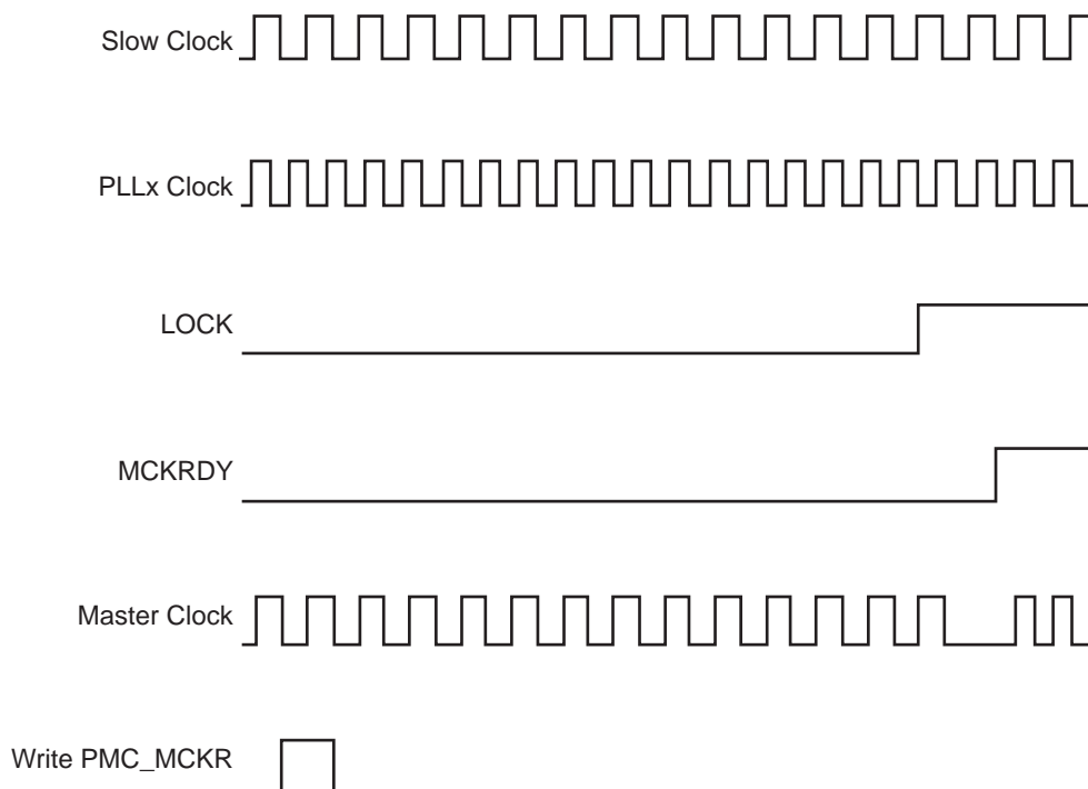
Figure 24-5. Switch Master Clock from Slow Clock to PLLx Clock
