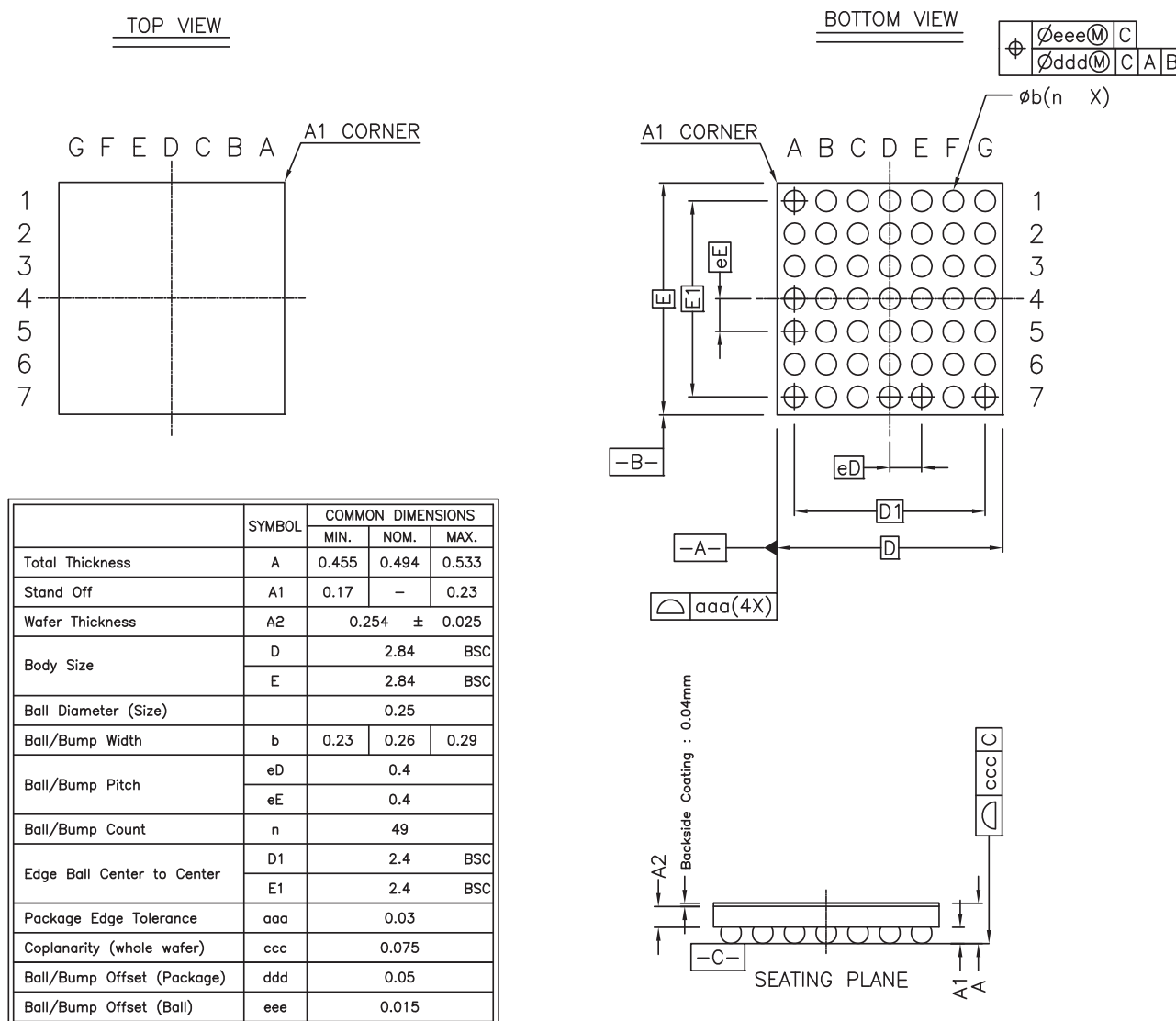
Figure 35-1. 49-lead WLCSP Package Mechanical Drawing
