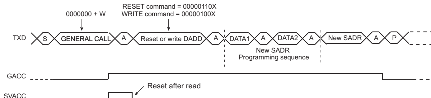
Figure 29-27. Master Performs a General Call
