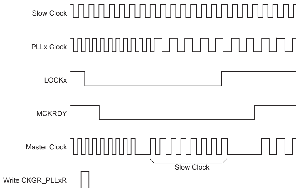
Figure 24-7. Change PLLx Programming
