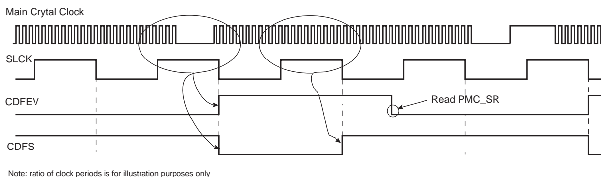
Figure 24-4. Clock Failure Detection (Example)
