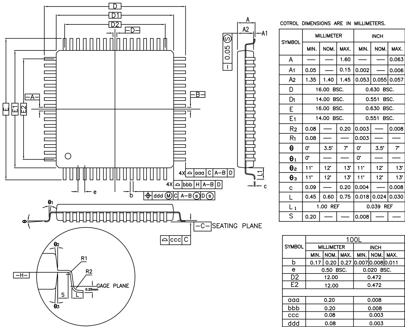
Figure 35-2. 100-lead LQFP Package Mechanical Drawing
