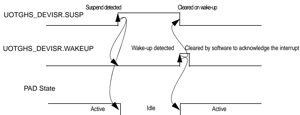
Figure 39-9. Pad Events
