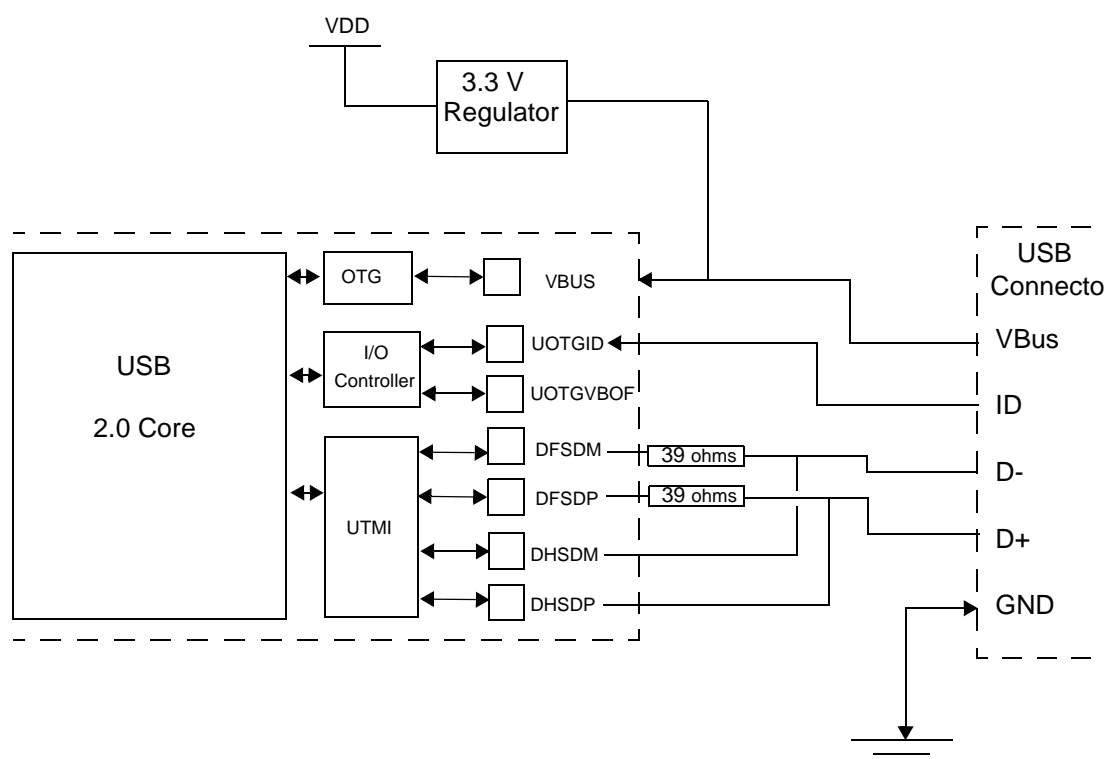
Figure 39-2. Bus-Powered Device Application Block Diagram
