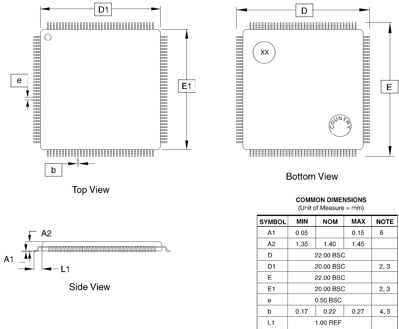
Figure 46-3. 144-lead LQFP Package Drawing
