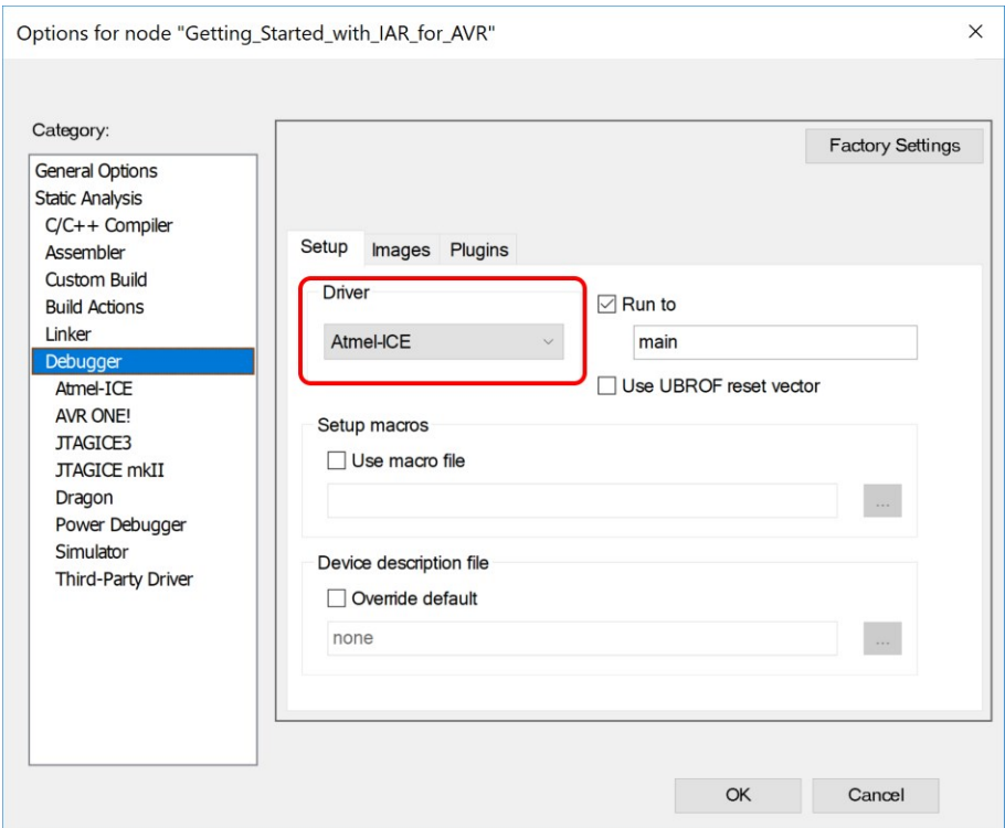
Figure 7-9. Select Debugger
