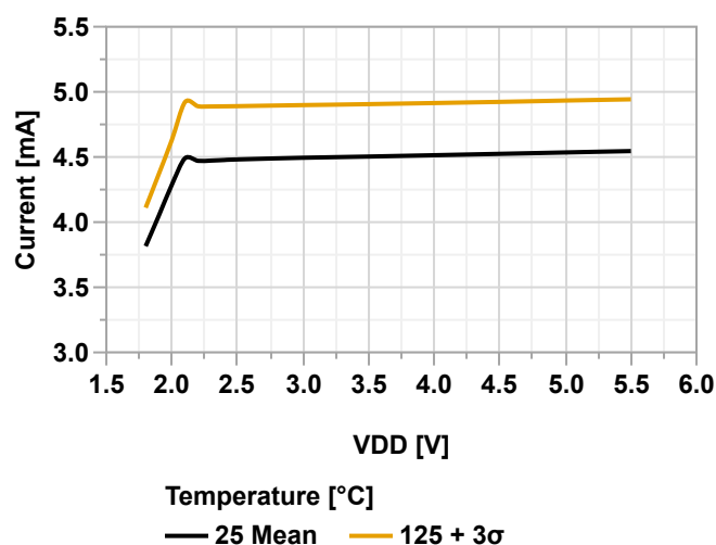
Figure 38-4. Active Power Consumption vs. V_{DD} (MCLKCTRLA.CLKSEL = OSCF, OSCF = 24 MHz)
