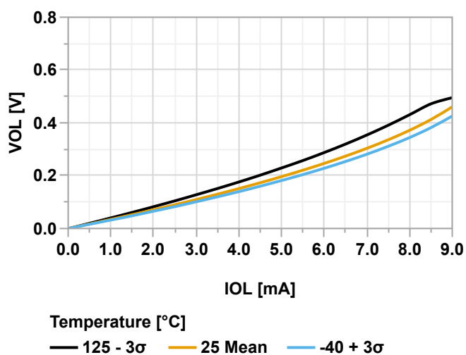
Figure 38-82. Output Pin - Maximum V_{OL} vs. Current, V_{DD} = 1.8V
