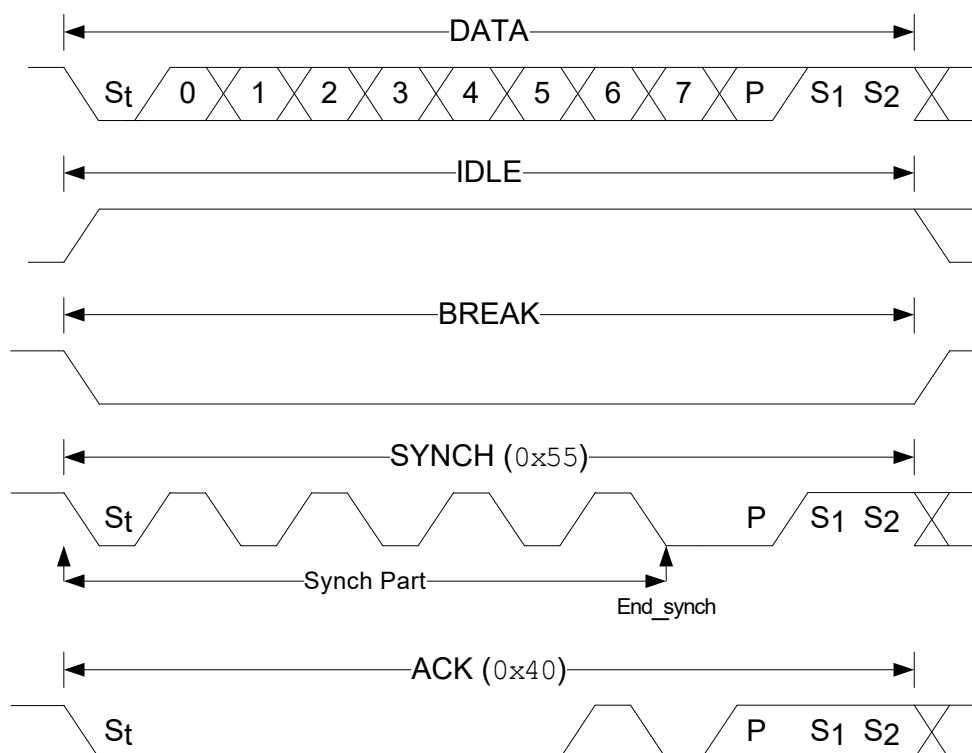
Figure 35-4. Supported UPDI Frame Formats
