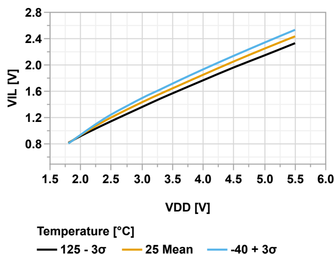
Figure 38-75. Input Pin with I 2 C Trigger - Maximum V_{IL} vs. V_{DD}
