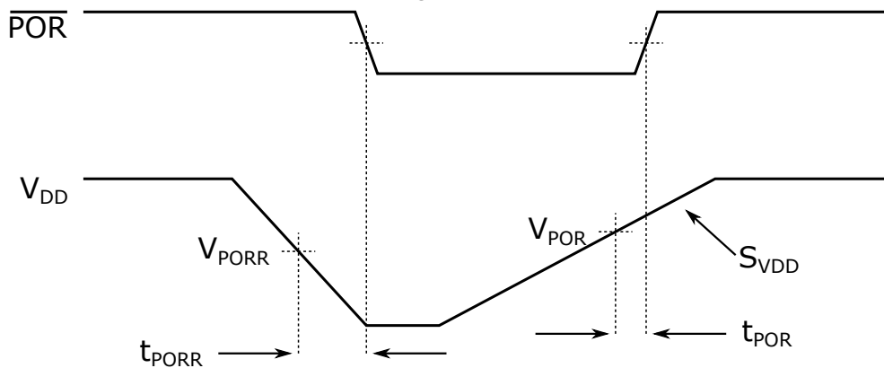
Figure 37-1. \overline{\text{POR}} and \text{POR} Re-Arm with Slow Rising V_{\text{DD}}
