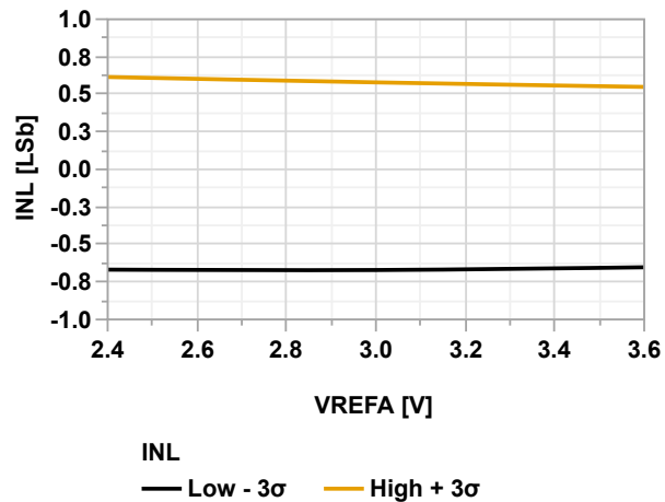
Figure 38-133. INL vs. V_{\text{REFA}} (ADC Differential Mode @60 kps, V_{\text{DD}} = 3.6\text{V} , T = 85^\circ\text{C} )
