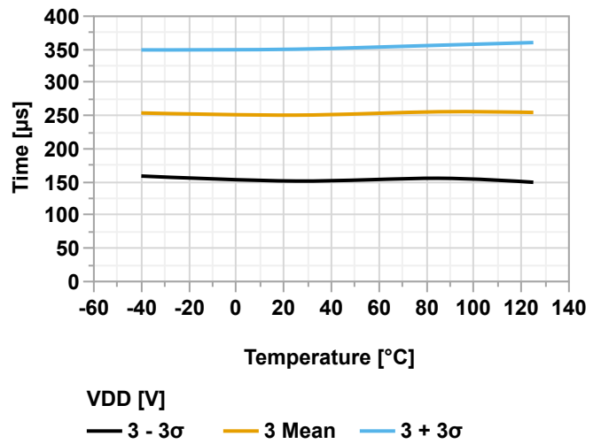
Figure 38-157. Settling Time vs. Temperature ( V_{\text{REFA}} = V_{\text{DD}} = 3.0\text{V} , Output Switch from 0\times3FF to 0\times000 )
