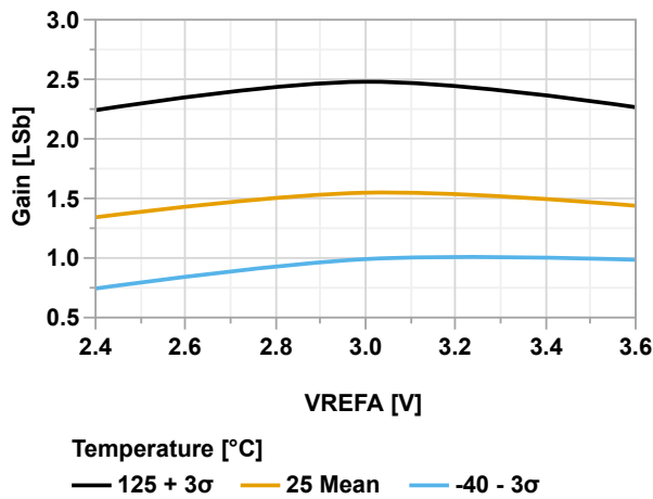
Figure 38-121. Positive Gain Error vs. V_{\text{REFA}} (ADC Differential Mode @60 kps, V_{\text{DD}} = 3.6\text{V} )
