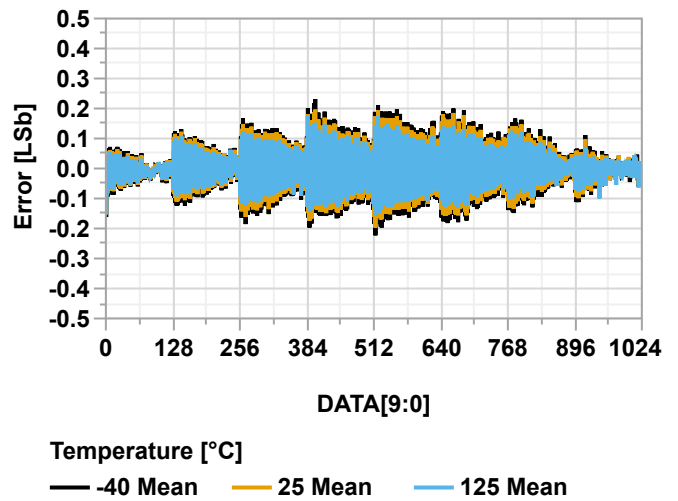
Figure 38-153. DNL vs. DAC Code ( V_{\text{REFA}} = V_{\text{DD}} = 5.5\text{V} )
