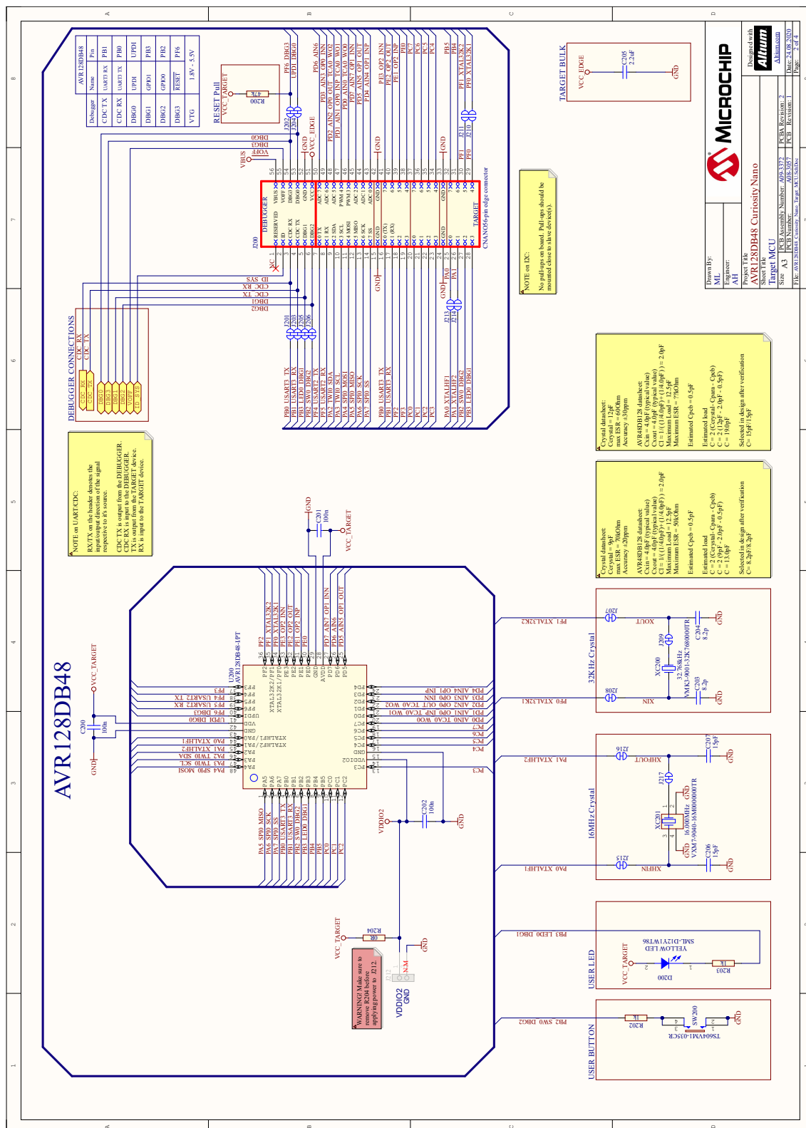
Figure 8-1. AVR128DB48 Curiosity Nano Schematic
