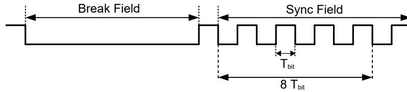
Figure 23-9. Auto-Baud Timing
