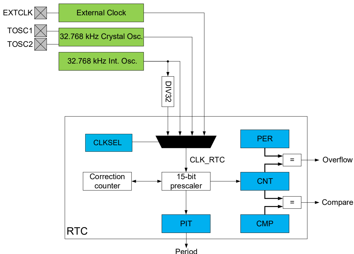
Figure 23-1. Block Diagram
