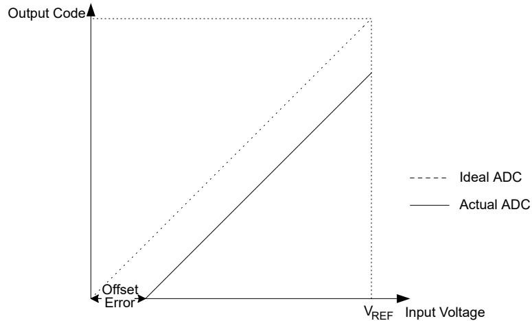
Figure 5-1. Offset Error
