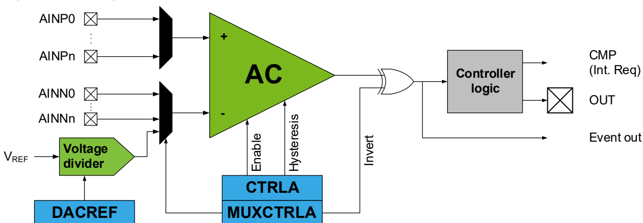
Figure 29-1. Analog Comparator
