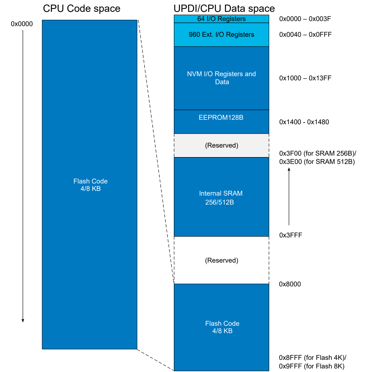
Figure 6-1. Memory Map
