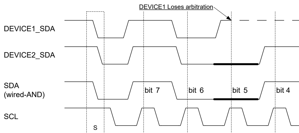
Figure 26-7. TWI Arbitration
