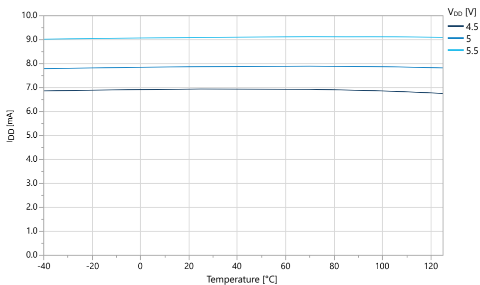
Figure 38-3. Active Supply Current vs. Temperature (f = 16 MHz OSC20M)
