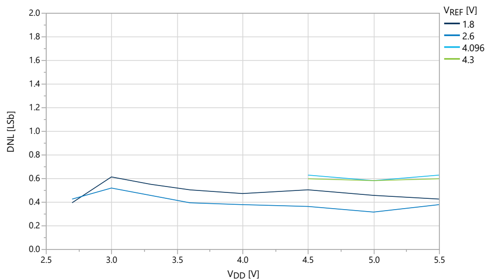
Figure 38-48. DNL vs. V_{DD} ( f_{ADC} = 115 ksp/s, T = 25^\circ C , REFSEL = External Reference)
