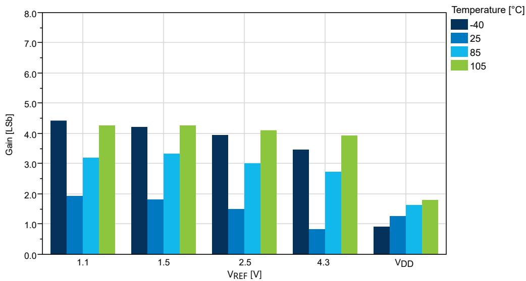
Figure 36-46. Gain Error vs. V_{REF} ( V_{DD} = 5.0\text{V} , f_{ADC} = 115 ksp/s), REFSEL = Internal Reference
