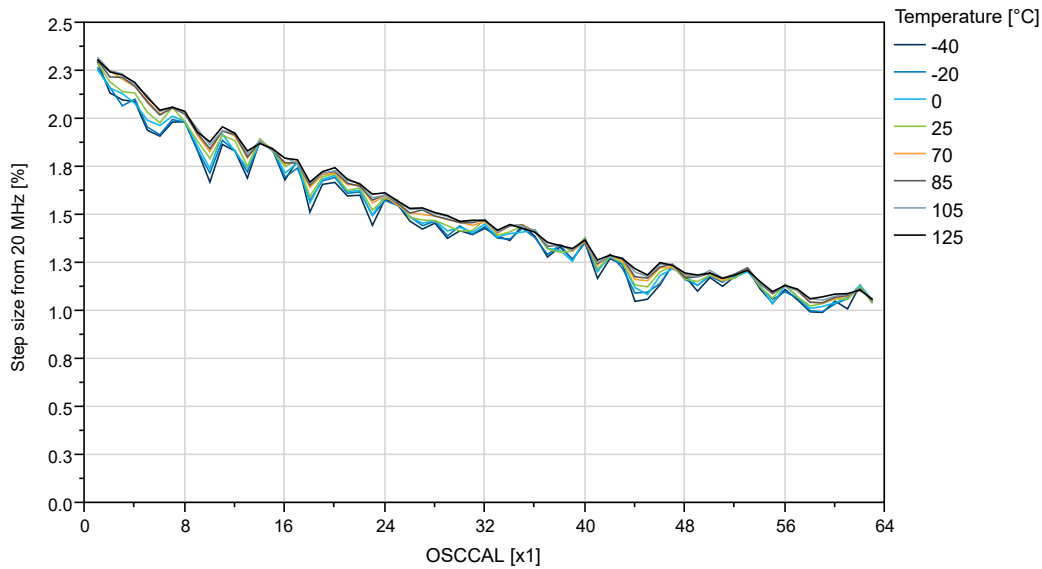
Figure 36-60. OSC20M Internal Oscillator: Calibration Stepsize vs. Calibration Value ( V_{DD} = 3V )
