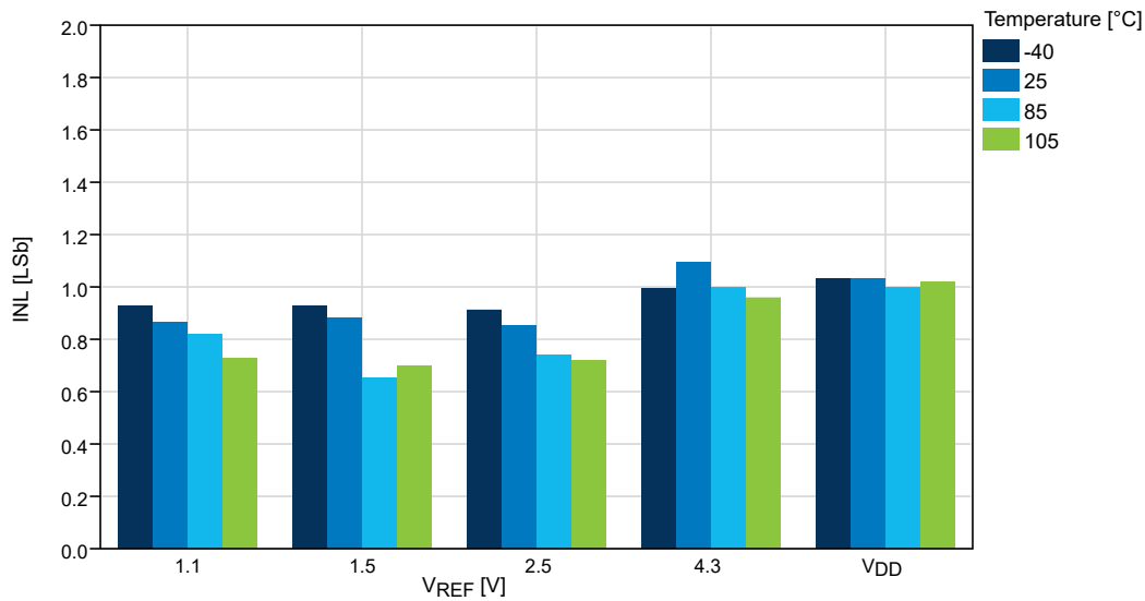
Figure 36-48. INL vs. V_{REF} ( V_{DD} = 5.0 V, f_{ADC} = 115 kps), REFSEL = Internal Reference
