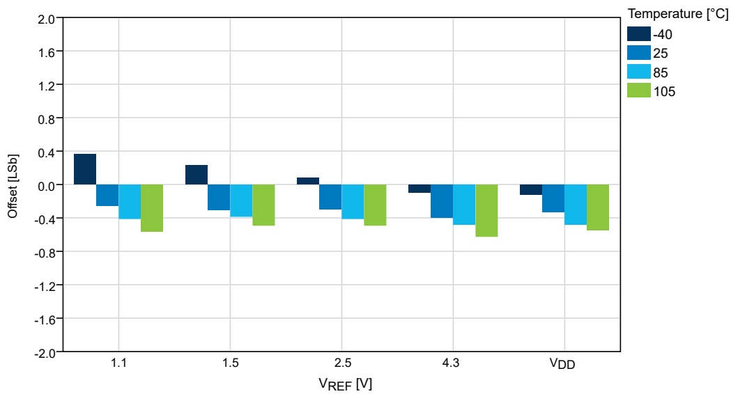
Figure 36-50. Offset Error vs. V_{REF} ( V_{DD} = 5.0 V, f_{ADC} = 115 kps), REFSEL = Internal Reference
