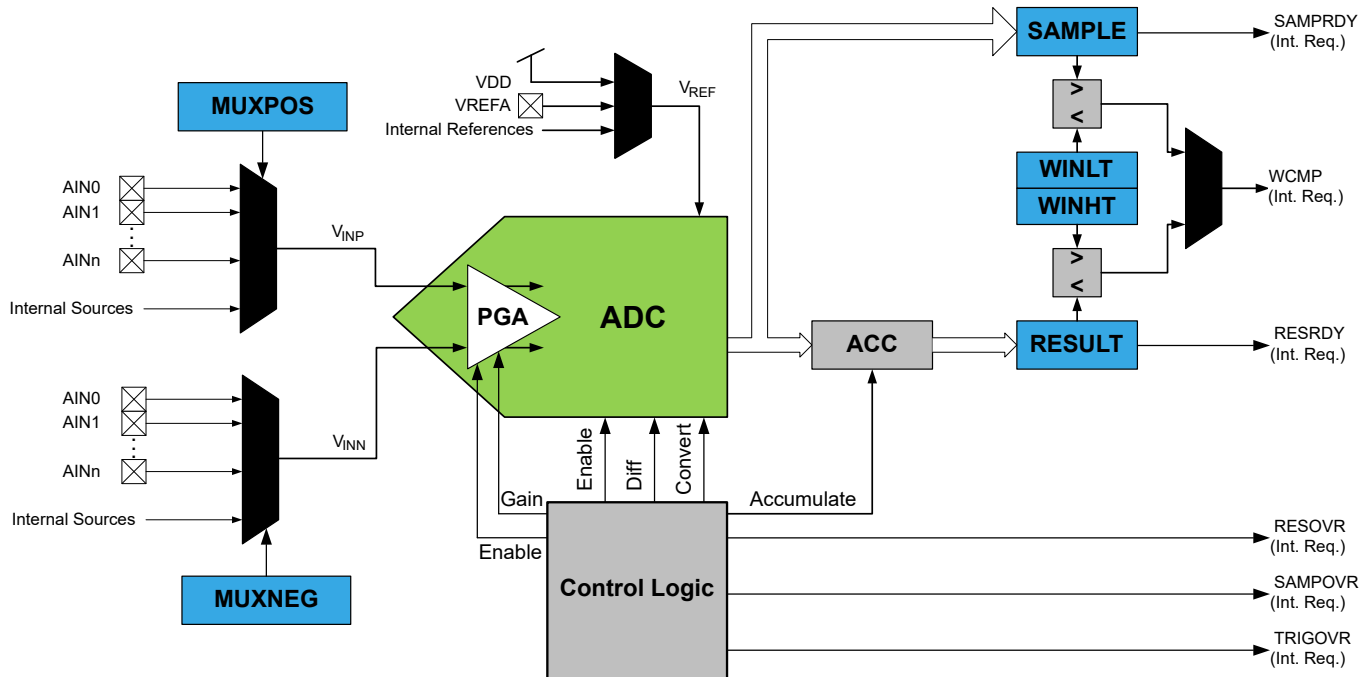
Figure 30-1. Block Diagram
