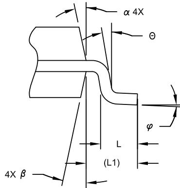
VIEW C
