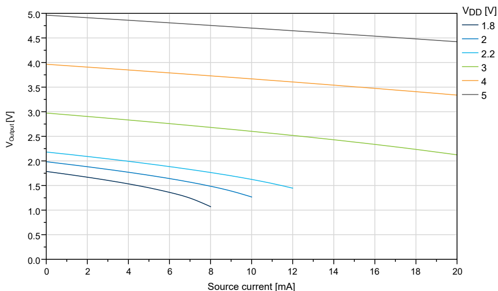
Figure 37-27. I/O Pin Output Voltage vs. Source Current ( T = 25^{\circ}\text{C} )
