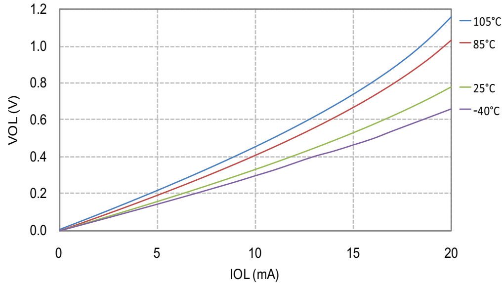
Figure 31-69. ATmega168PB: I/O Pin Output Voltage vs. Sink Current ( V_{CC} = 3V )
