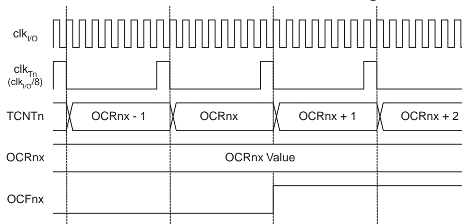
Figure 17-11. Timer/Counter Timing Diagram, Setting of OCF1x, with Prescaler ( f_{\text{clk\_I/O}}/8 )
