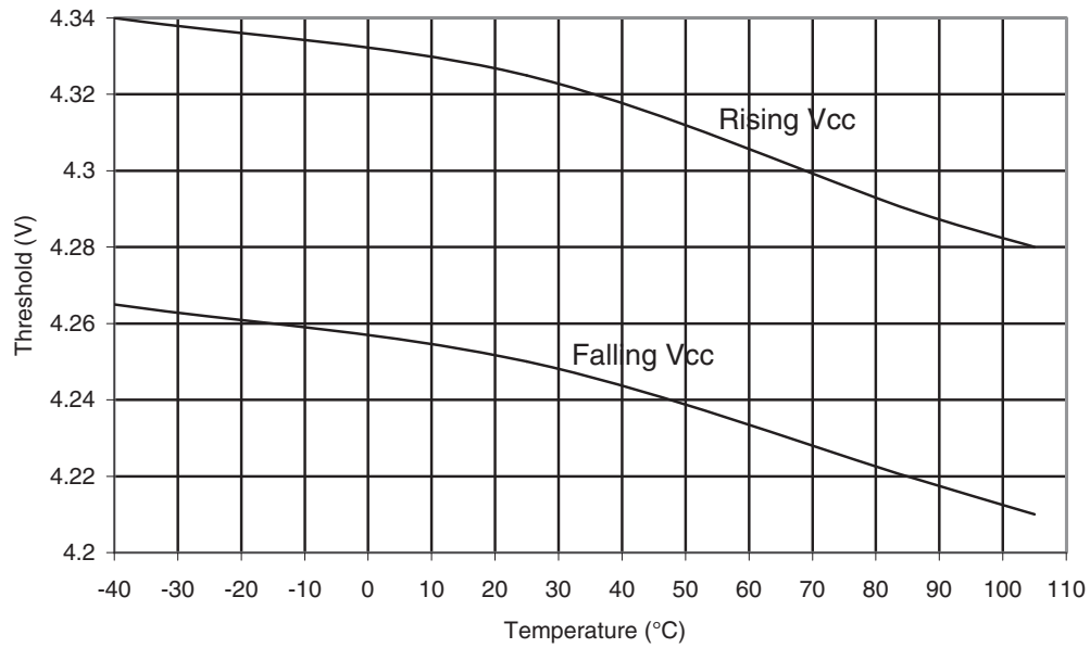
Figure 32-32.ATmega48PA: BOD Thresholds vs. Temperature (BODLEVEL is 4.3V)
