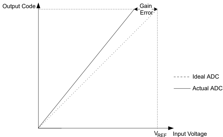
Figure 5-2. Gain Error
