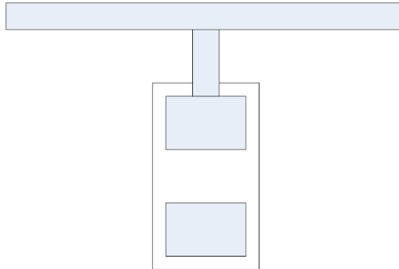
Figure 11-4. Incorrect Stub Route to Capacitor Pad
