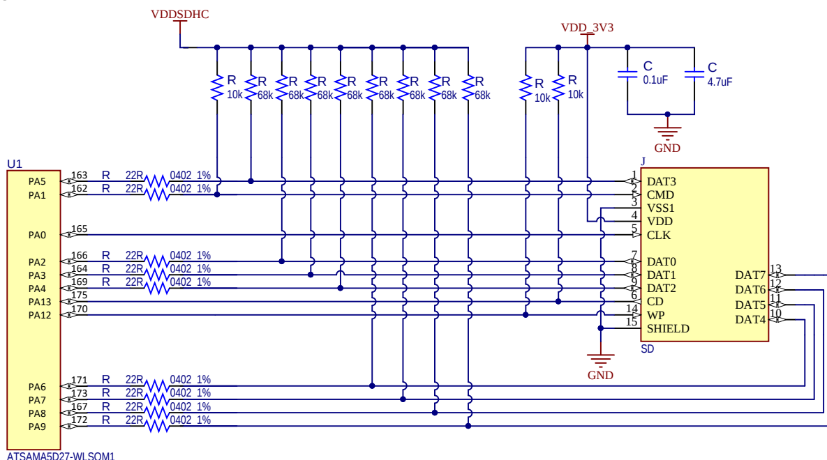
Figure 4-21. 8-bit SD Card Interface Example Schematic
