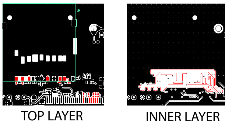
Figure 4-23. EMI Improvement Layout Example
