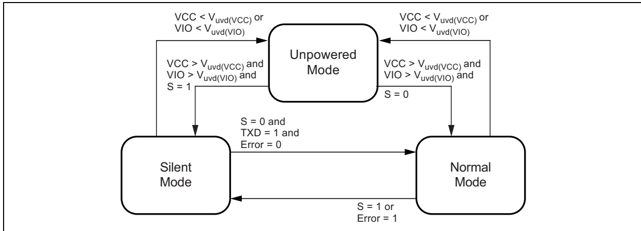
FIGURE 1-1: OPERATING MODES
