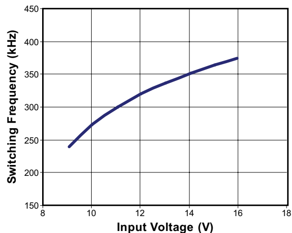
Fig. 5. Switching Frequency vs. Input Voltage Plot (Full Load)
