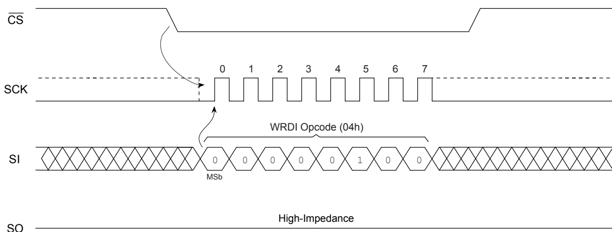
Figure 6-3. WRDI Timing
