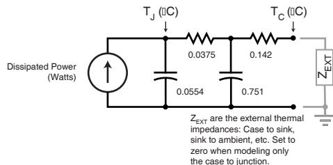
FIGURE 2, TRANSIENT THERMAL IMPEDANCE MODEL
