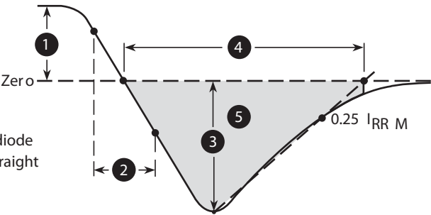
Figure 10. Diode Reverse Recovery Waveform Definitions
