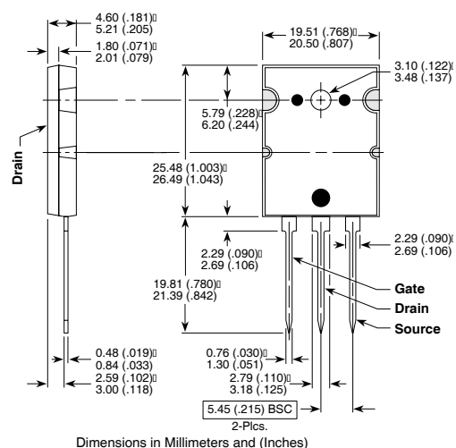
TO-264 (L) Package Outline
