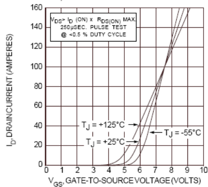
FIGURE 4, TRANSFER CHARACTERISTICS
