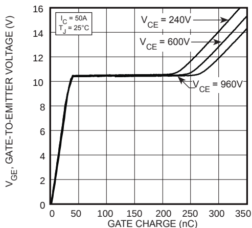
FIGURE 4, Gate charge
