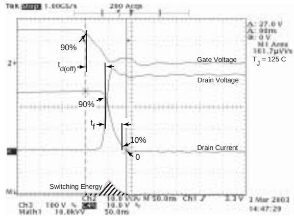
Figure 19, Turn-off Switching Waveforms and Definitions
