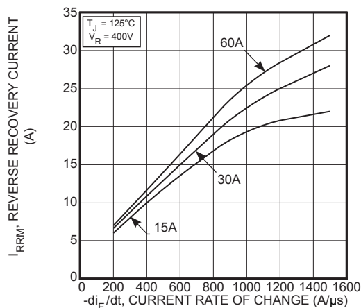
Figure 26. Reverse Recovery Current vs. Current Rate of Change
