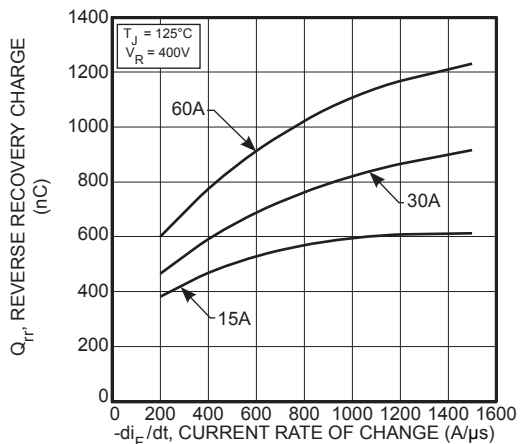
Figure 25. Reverse Recovery Charge vs. Current Rate of Change
