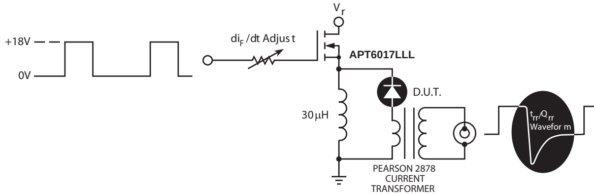
Figure 30. Diode Test Circuit
