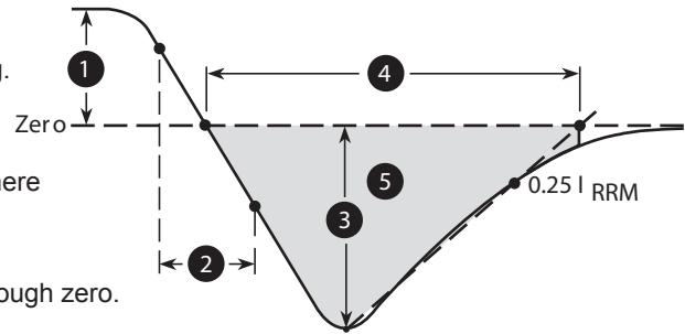
Figure 31. Diode Reverse Recovery Waveform Definition
