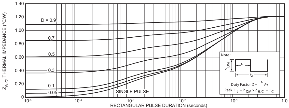
FIGURE 22, MAXIMUM EFFECTIVE TRANSIENT THERMAL IMPEDANCE, JUNCTION-TO-CASE vs. PULSE DURATION
