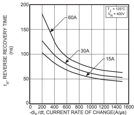
Figure 24. Reverse Recovery Time vs. Current Rate of Change
