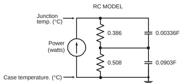
FIGURE 2, TRANSIENT THERMAL IMPEDANCE MODEL
