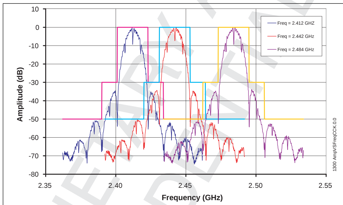
Figure 10: 802.11b Spectrum Mask at 23.5 dBm, Total Current 220 mA
