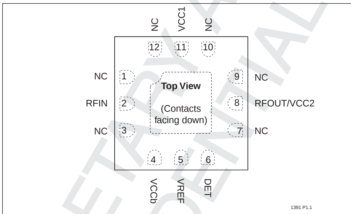
Figure 2: Pin Assignments for 12-contact XQFN
