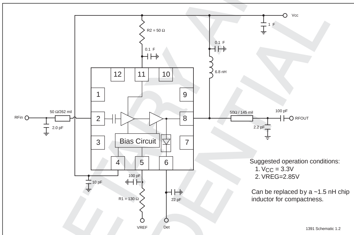
Figure 11: Typical Schematic for High-Power/High-Efficiency 802.11b/g Applications
