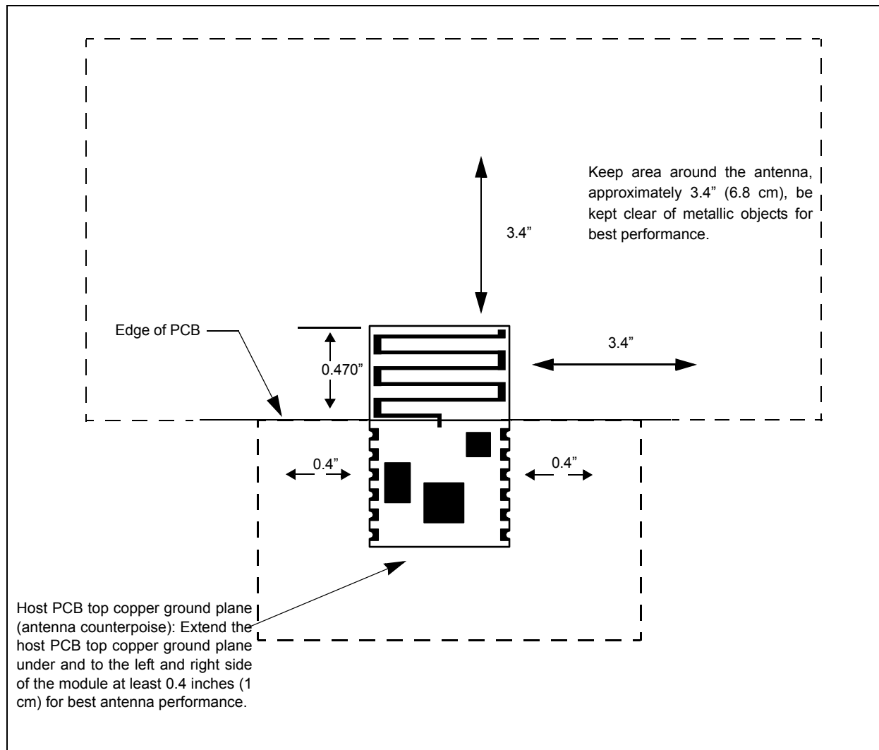
FIGURE 1-5: MOUNTING DETAILS
