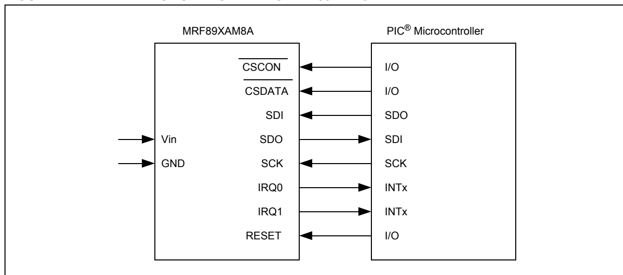
FIGURE 1-2: MICROCONTROLLER TO MRF89XAM8A INTERFACE
