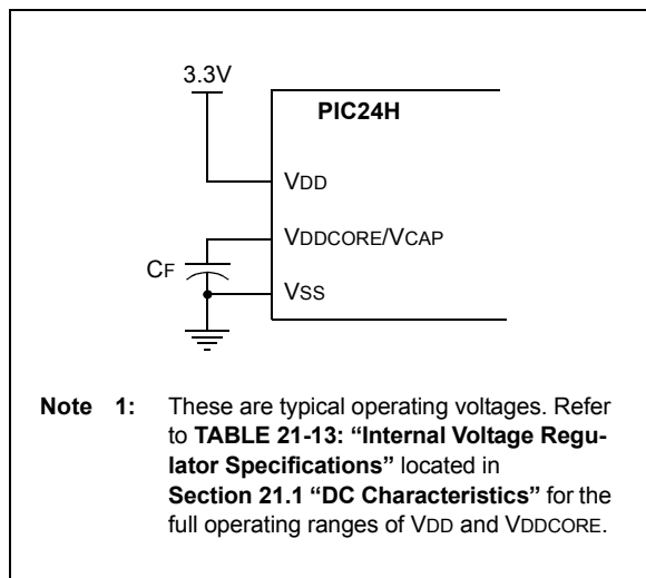
FIGURE 18-1: CONNECTIONS FOR THE ON-CHIP VOLTAGE REGULATOR (1)
