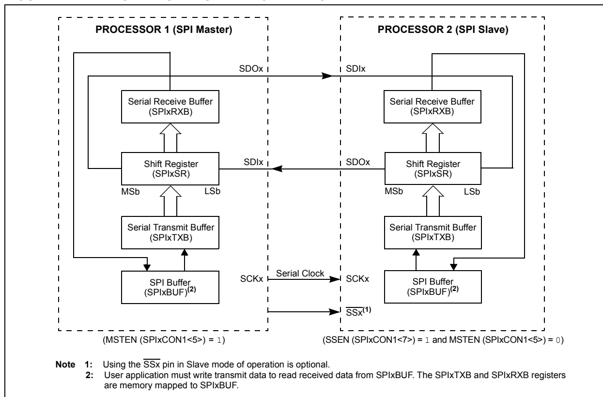
FIGURE 14-2: SPI MASTER/SLAVE CONNECTION
