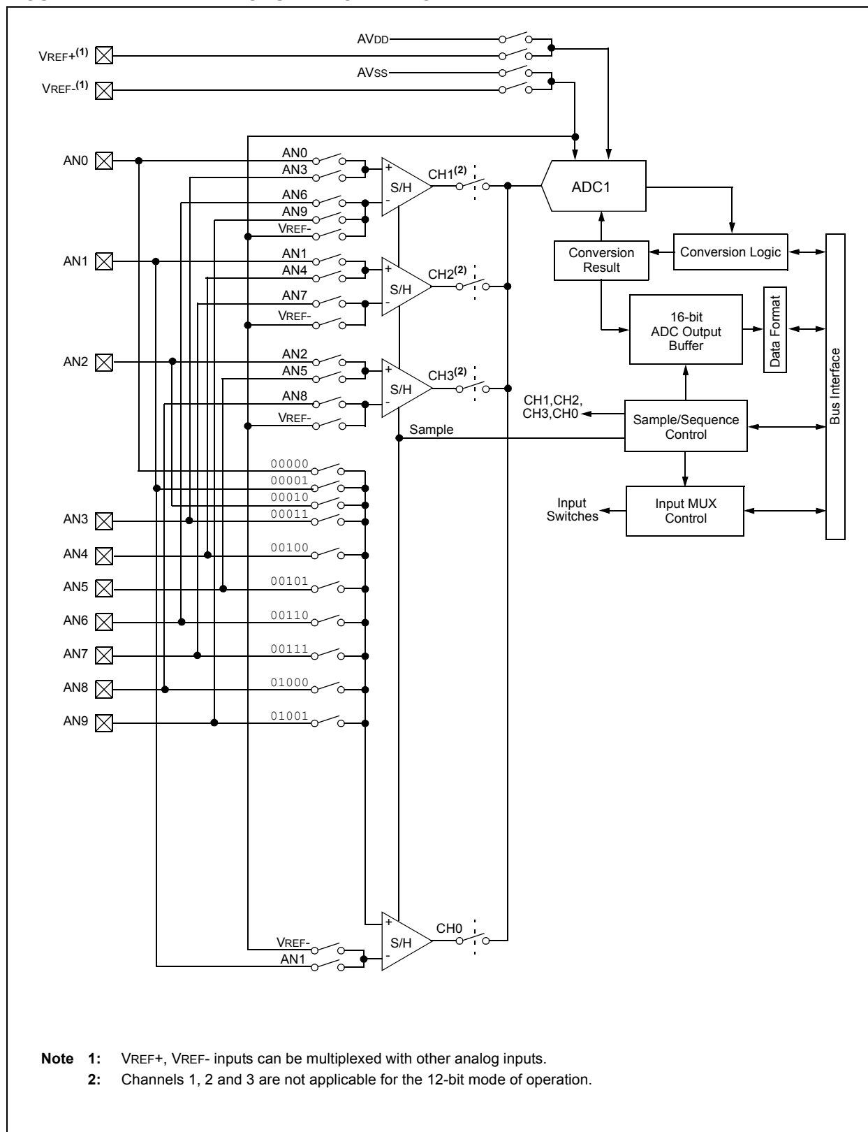
FIGURE 17-1: ADC1 MODULE BLOCK DIAGRAM
