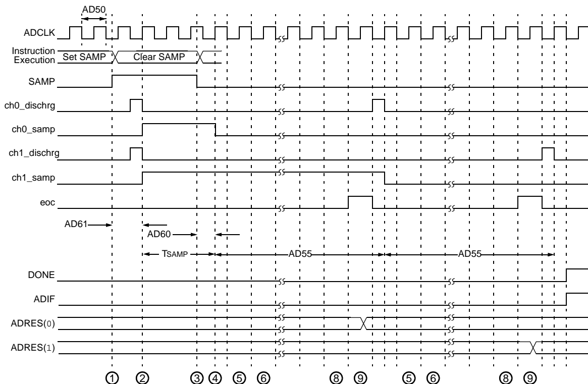
FIGURE 24-25: 10-BIT HIGH-SPEED A/D CONVERSION TIMING CHARACTERISTICS (CHPS<1:0> = 01, SIMSAM = 0, ASAM = 0, SSRC<2:0> = 000)
