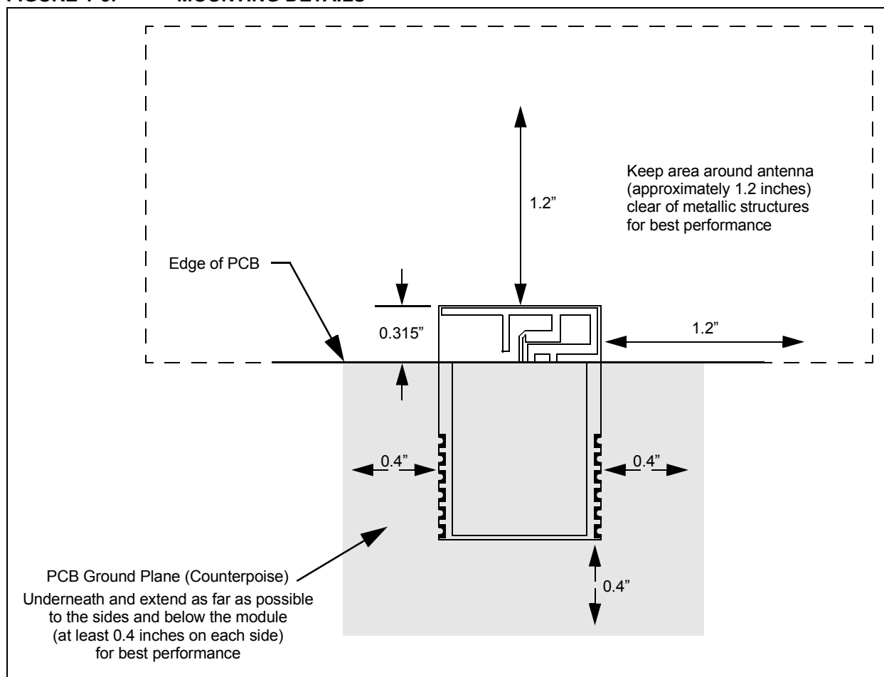
FIGURE 1-5: MOUNTING DETAILS
