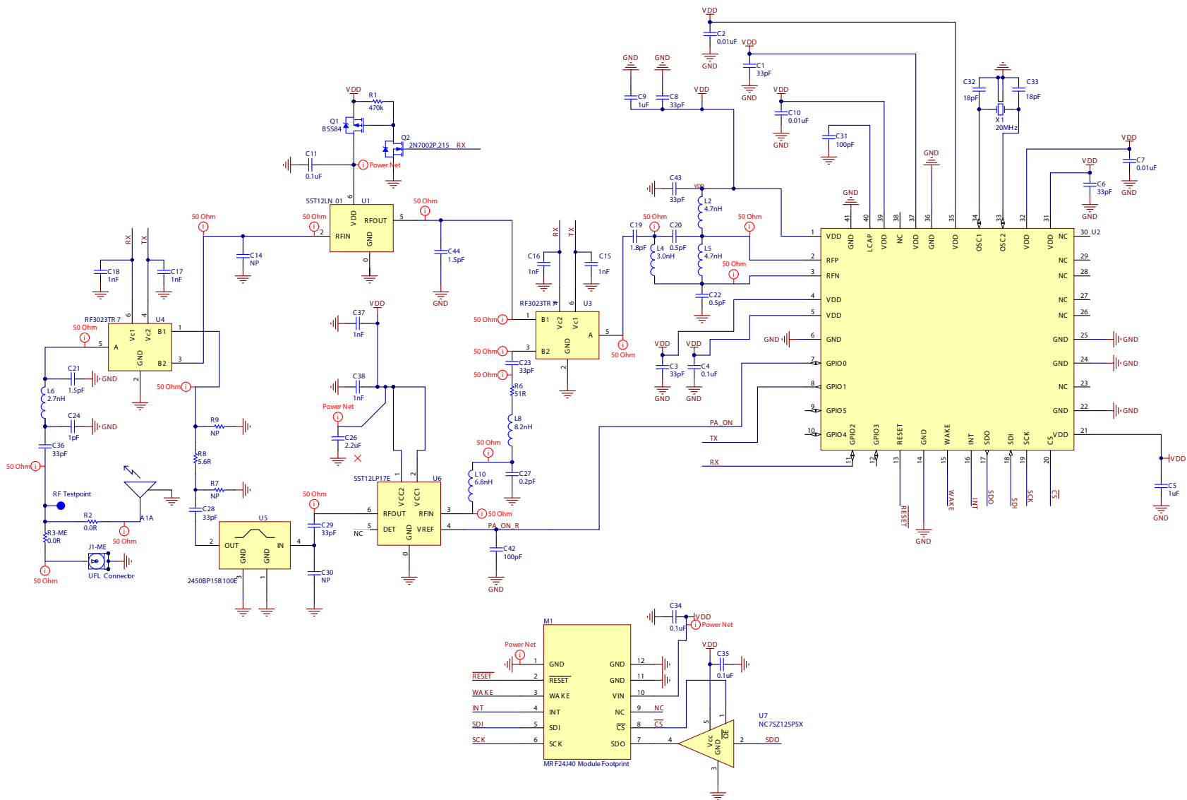
FIGURE 2-5: MRF24J40MD/ME SCHEMATIC
