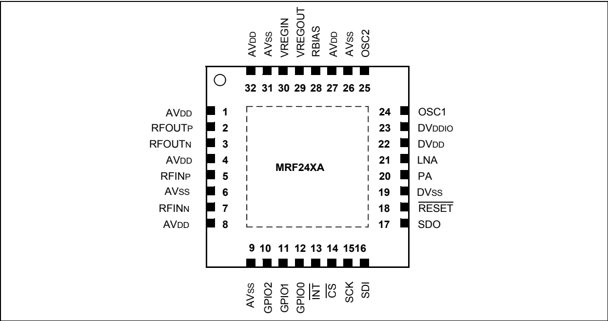
Pin Diagram
