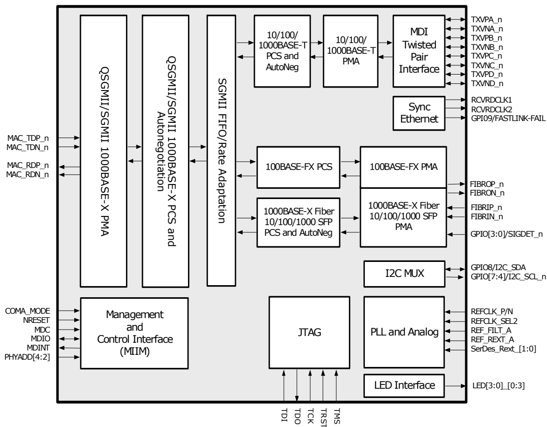
FIGURE 4: BLOCK DIAGRAM
