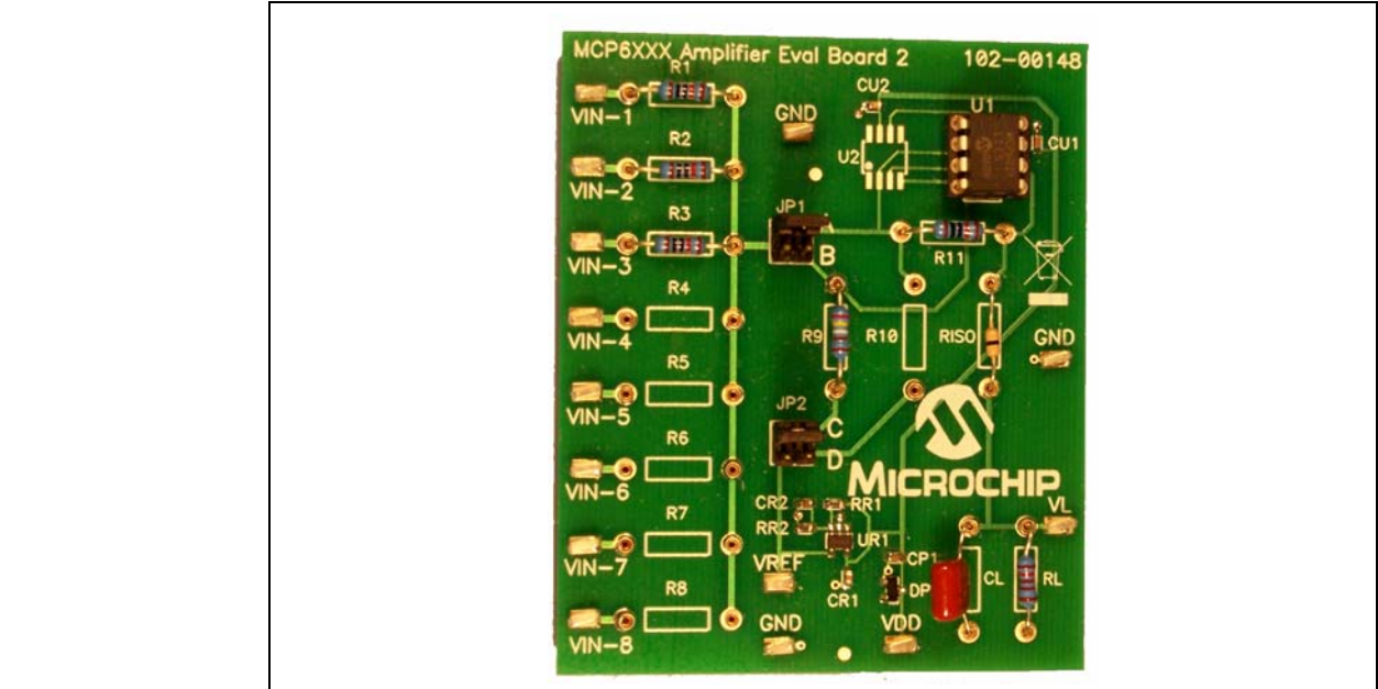
FIGURE 2-13: Picture of the Inverting Summing Amplifier Supported by the MCP6XXX Amplifier Evaluation Board 2.
