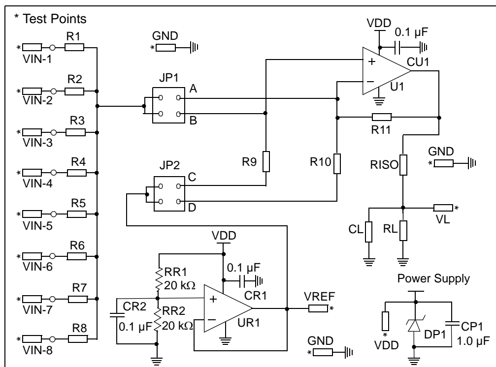
FIGURE 2-1: MCP6XXX Amplifier Evaluation Board 2 Circuit Diagram.
