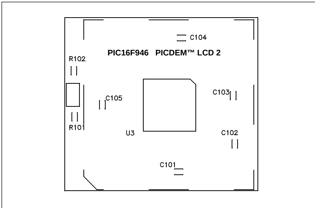
FIGURE A-18: PIC16F946 PIM LAYOUT
