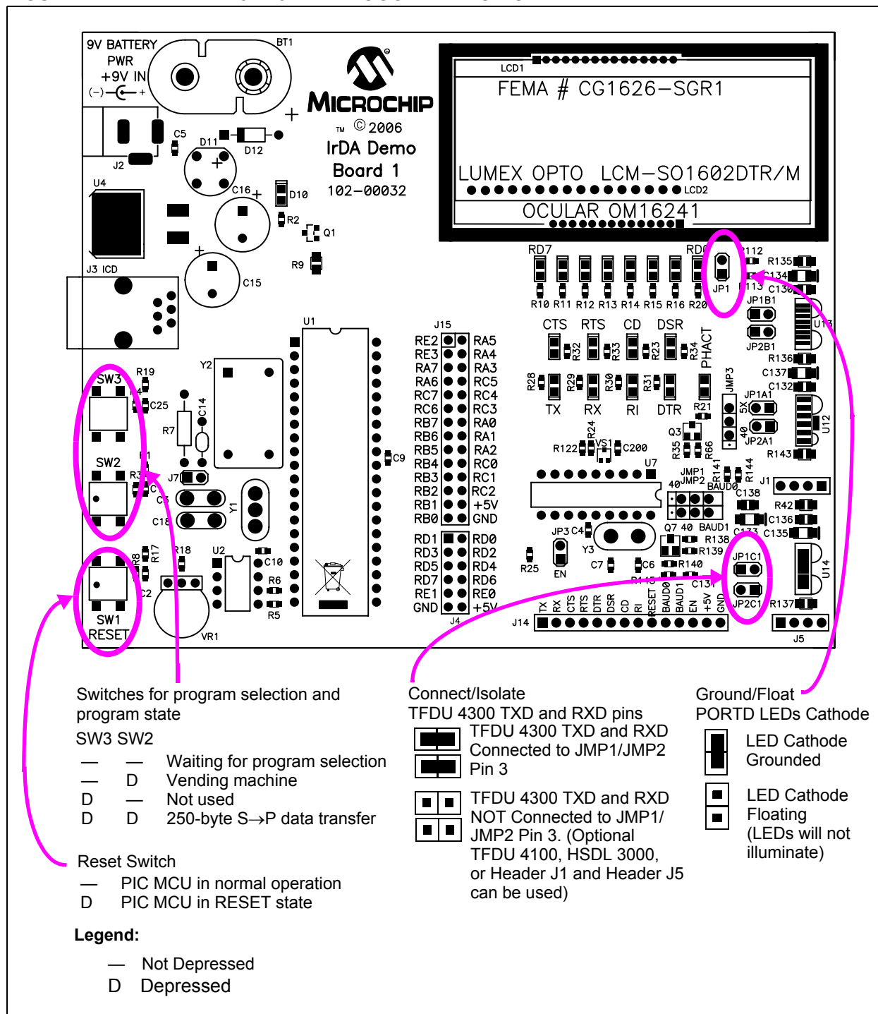
FIGURE 2-2: MCP215X/40 DATA LOGGER DEMO BOARD
