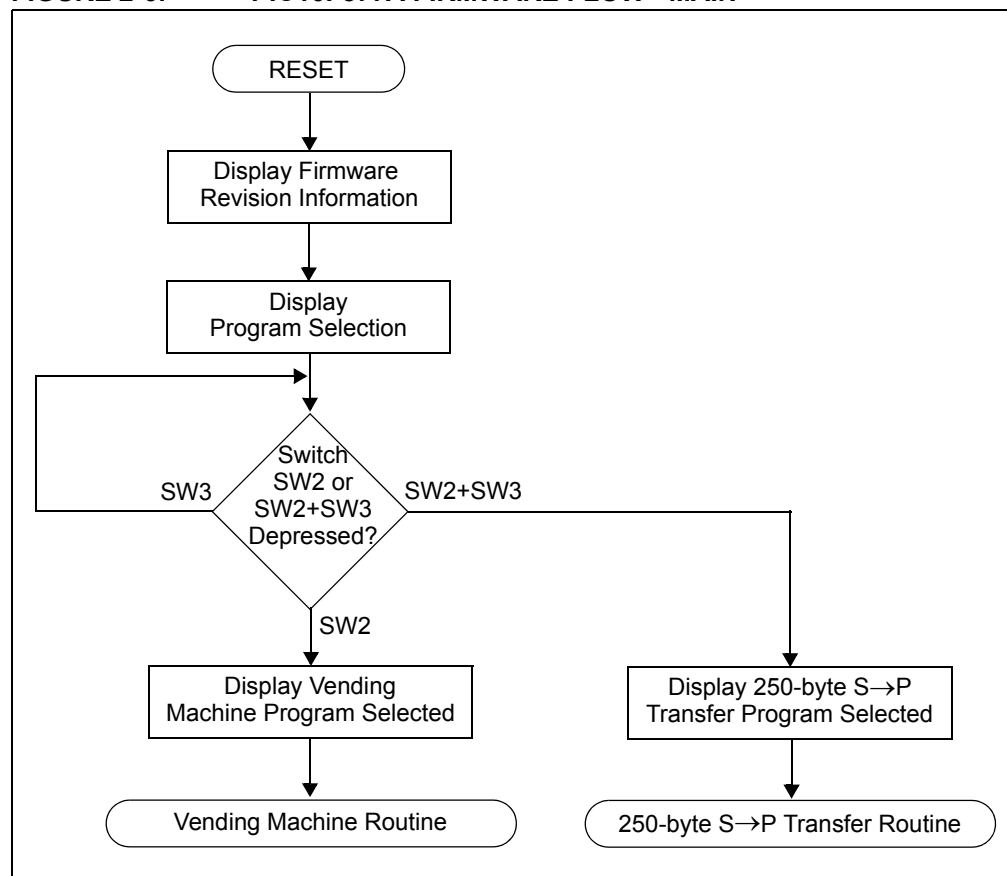
FIGURE 2-6: PIC16F877A FIRMWARE FLOW - MAIN
