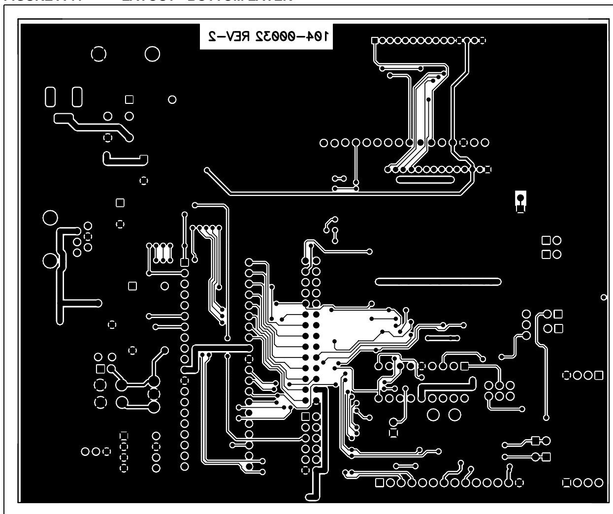
FIGURE A-7: LAYOUT - BOTTOM LAYER
