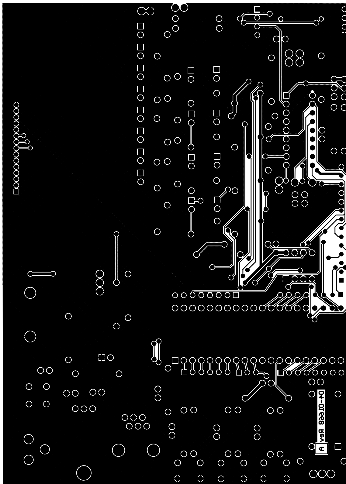
FIGURE A-10: MCP215X DATA LOGGER DEMO BOARD LAYOUT - BOTTOM LAYER — REV. 1
