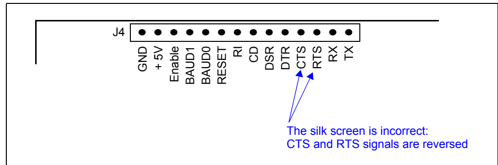
FIGURE F-4: SIGNAL INTERFACE HEADER J14
