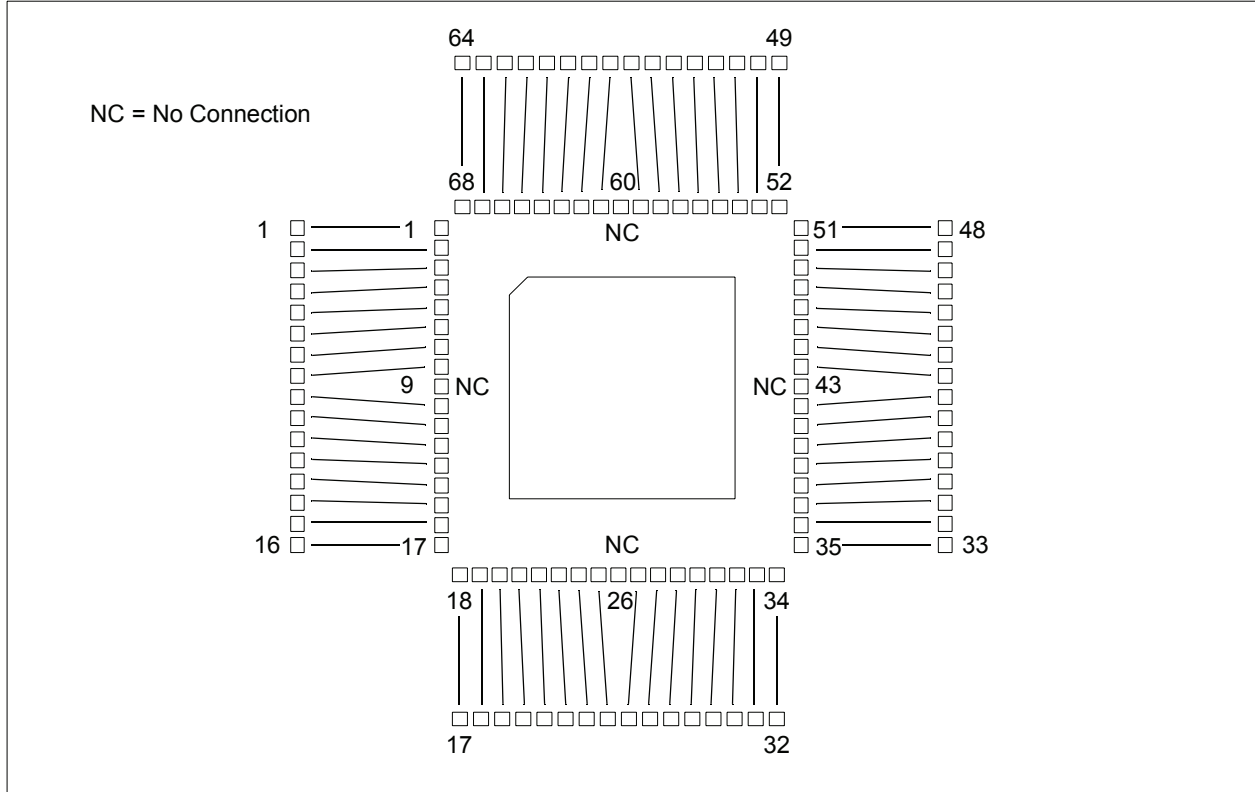
FIGURE 6-4: DVA-68PL TO 64-PIN TQFP
